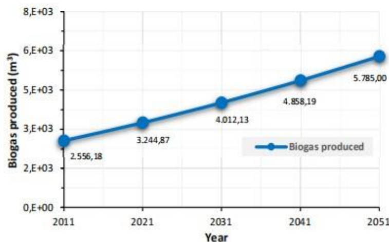
Figure 1: Biogas Generation.
