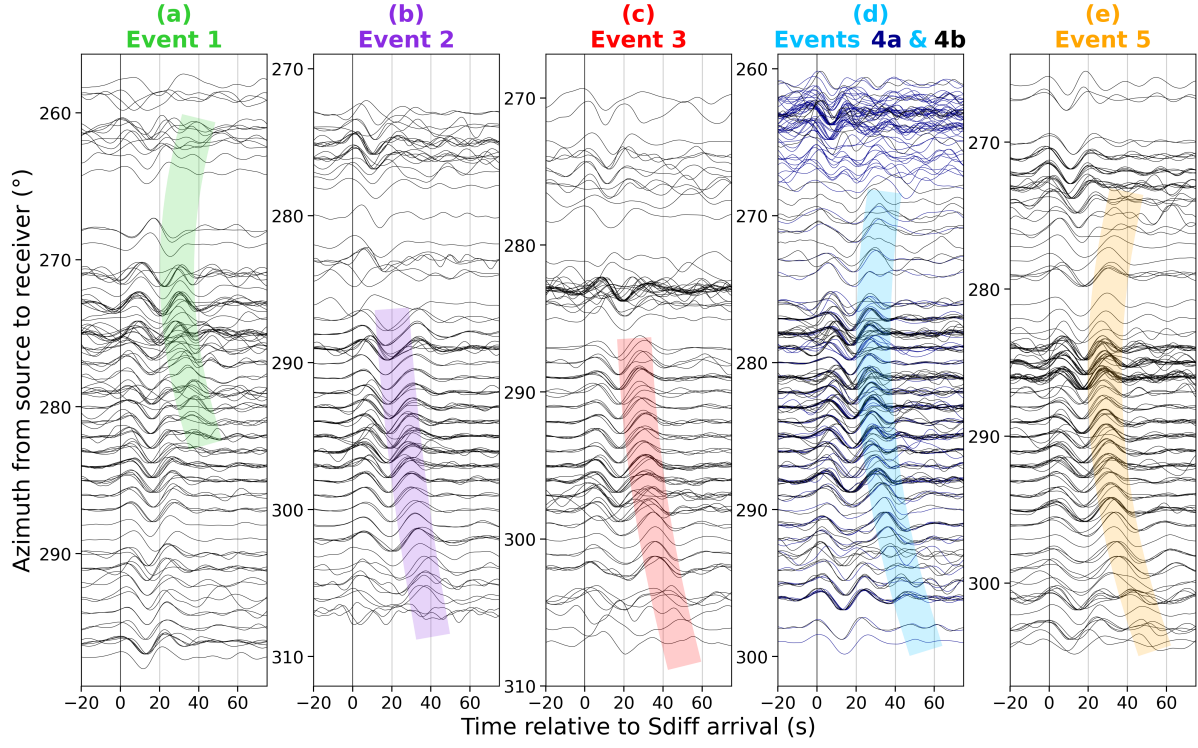
Figure S2. Same as Figure 4 but filtered between 20–30 s period.
