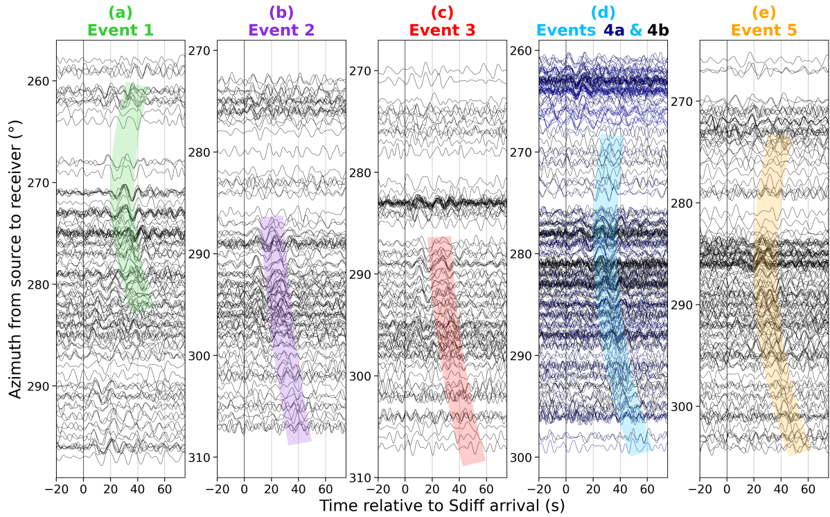
Figure S1. Same as Figure 4 but filtered between 7–12 s period.
