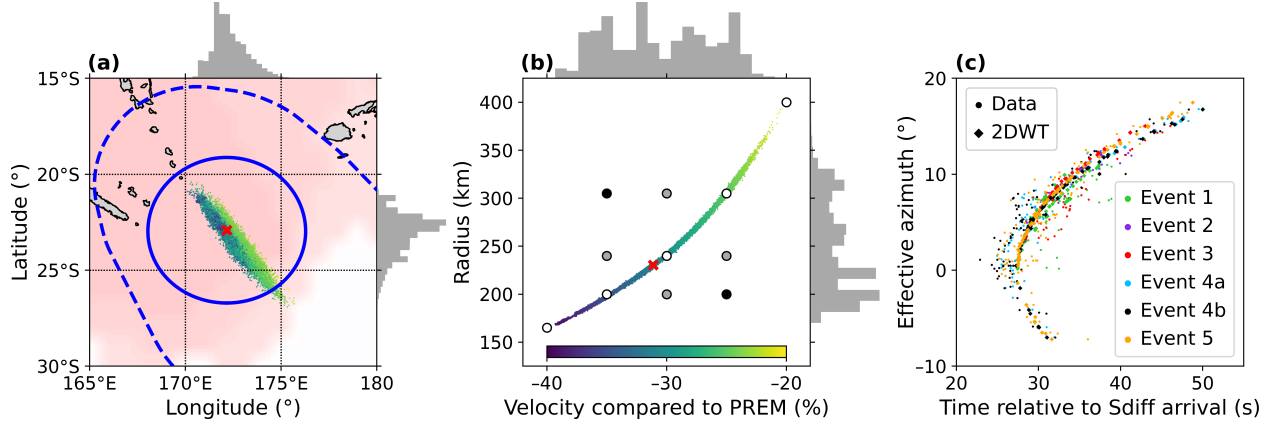
Figure 5. Ensemble of models that fit the Sdiff+ arrival times from the rj-McMC, showing the distribution of (a) midpoint locations and the (b) trade-off in ULVZ velocity reduction and radius. The median model is marked with a red cross and histograms of each of the parameters are projected onto the respective axes. The outline of the median model ( \sim 230 km radius and \sim 31\% velocity reduction, located at 172.2^\circ E and 22.9^\circ S) and convex hull of the ensemble parameter space are shown as solid and dashed blue lines, respectively (the full convex hull can be seen in Figures 1 & 3). Colours of model midpoints in (a) correspond to the velocity value of the ensemble model, which approximately corresponds to radius. The background in (a) corresponds to the LLVP vote map at 2800 km depth [Cottaar and Lekic, 2016]. Circles in (b) are parameters used for full waveform modelling of trade-offs (Figure S7 & Table S2). (c) Comparison of the Sdiff+ arrival times and the predicted data for the median model. Predicted arrival times for all models in (b) are shown in Figure S8.
