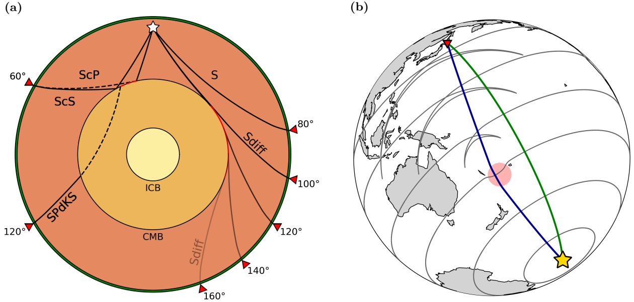
Figure 2. (a) Propagation of ScP, ScS, SPdKS, S, and Sdiff seismic phases from an earthquake (star) to receivers (triangles) through a cross-section of the Earth. ScP and ScS are core-reflected phase that sample bounce points on the CMB. SPdKS and Sdiff are phases that have diffracting legs along the CMB, with diffraction ray paths that attenuate with distance. (b) Wavefront propagation of Sdiff from an earthquake (star), calculated using the 2D wavefront tracker [Hauser et al., 2008; Martin et al., 2023a]. The wavefront propagates through time (sequential grey lines), producing postcursor signals as it passes across a ULVZ (pink circle). A receiver (triangle) detects the direct arrival (Sdiff, green line) and an additional delayed arrival due to refraction from the ULVZ (Sdiff+, blue line) at a different angle to the direct backazimuth.
