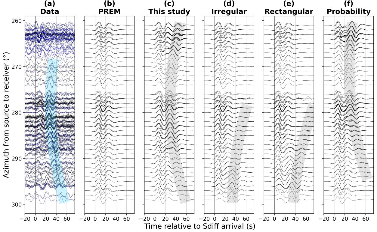
Figure 7. Waveform data and synthetics for the Vanuatu ULVZ in this study and for other models of proximate ULVZs. (a) Observed and (b-f) synthetic displacement waveforms for Events 4a & 4b. Synthetics for PREM with (b) no ULVZ, (c) the preferred ULVZ in this study, (d) the irregularly shaped Samoa ULVZ [Thorne et al., 2021], (e) the rectangular-shaped Samoa ULVZ [Krier et al., 2021], and (f) a ULVZ with parameters of our preferred model located at the proximate probability peak of Thorne et al. [2021] (Figure S15). The Sdiff+ signals are highlighted where visible. Data are filtered between 10–20 s period.
