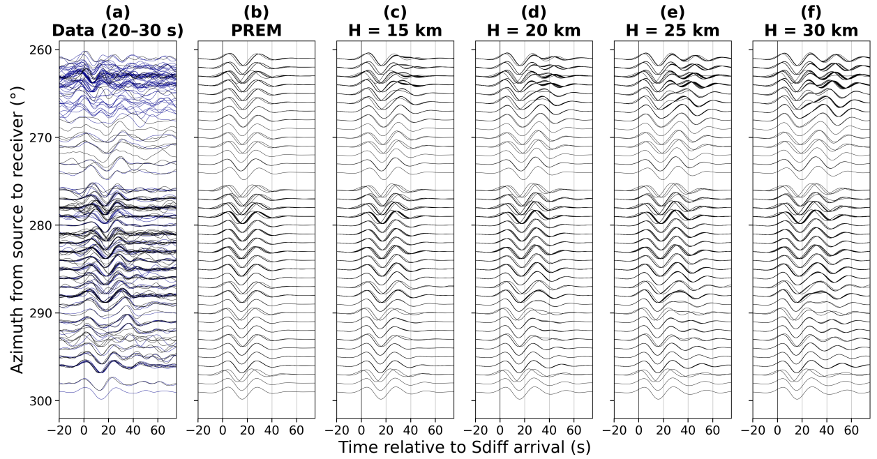
Figure S10. Same as Figure S9 but filtered between 20–30 s period.
