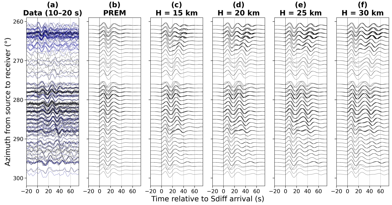
Figure S9. (a) Real data and synthetic waveforms for (b) PREM with no ULVZ and PREM with a cylindrical ULVZ of height (c) 15 km, (d) 20 km, (e) 25 km, and (f) 30 km for Events 4a & 4b, filtered between 10–20 s period. All models use dVs of -30% and a radius of 240 km (Model A3, Table S2).
