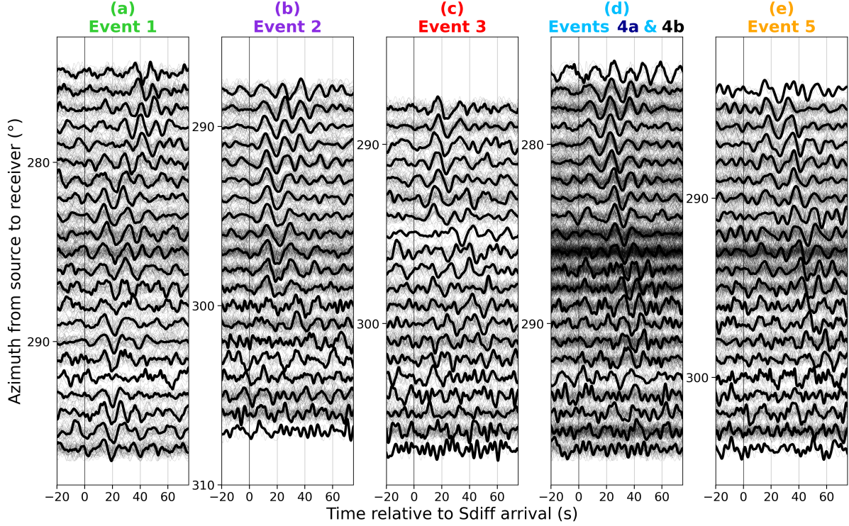
Figure S4. Displacement waveforms from the short period Hi-net seismometers for Events 1–5 filtered between 10–20 s period. The linear stack of each 1° azimuthal bin (thick black lines) overlay the individual seismograms (thin grey lines). Note the different (y axis) azimuthal range compared to broadband data.
