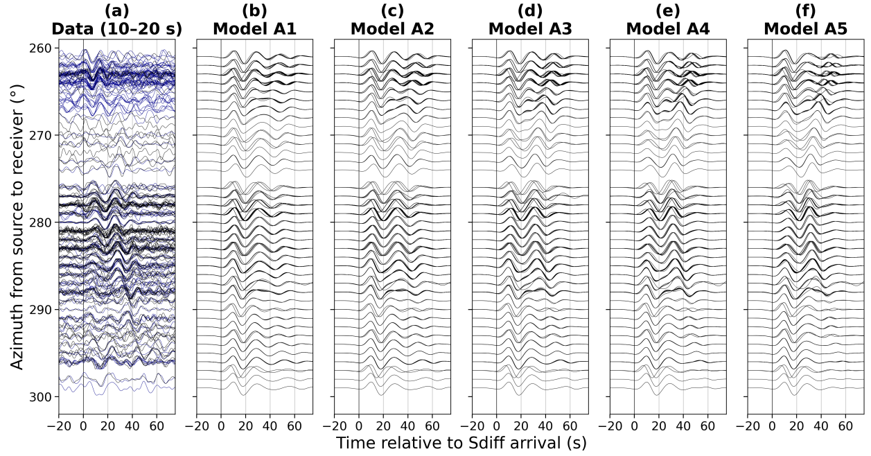
Figure S11. (a) Real data and (b-f) synthetic waveforms for PREM with a cylindrical ULVZ with parameters corresponding to Table S2. Model A parameters correspond to on the trade-off curve from the 2DWT inversion ensemble (white circles, Figure S7). Data are filtered between 10–20 s period.
