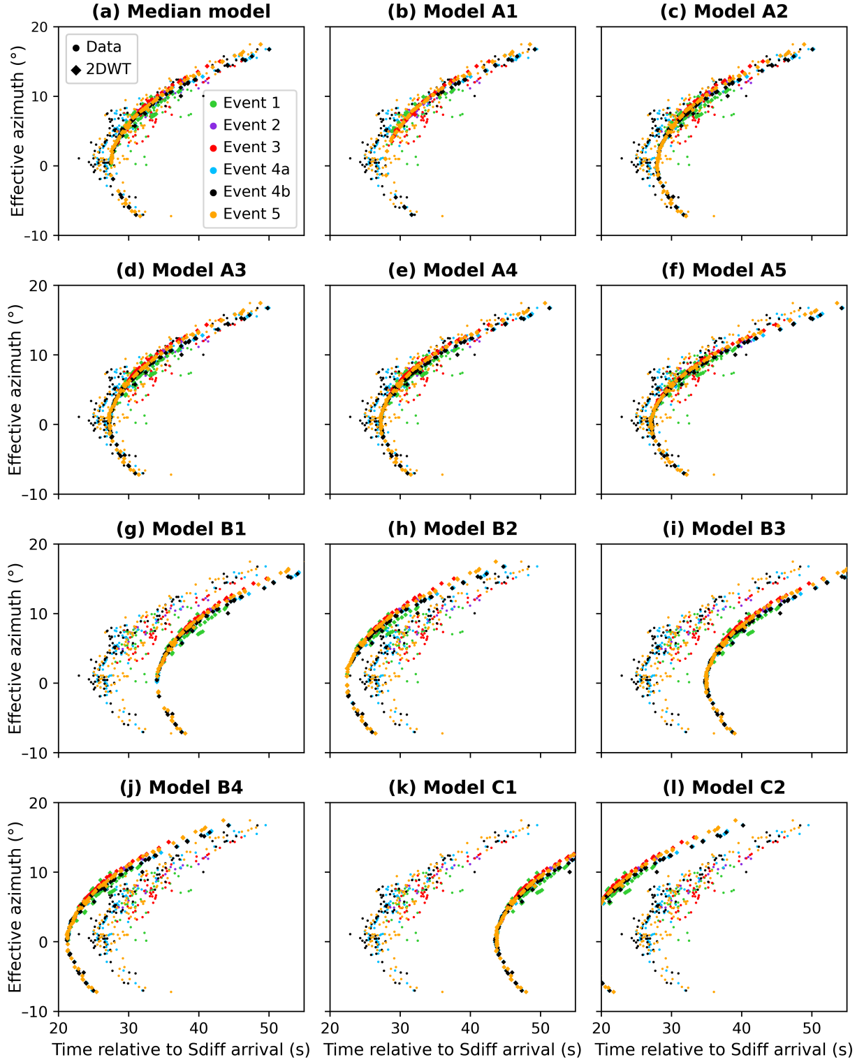
Figure S8. Predicted travel times from the 2DWT for the various models for which we compute full waveform synthetics (Figure S7 & Table S2). (a) is the same as Figure 5c. Note that the 2DWT predictions do not account for height of the model.
