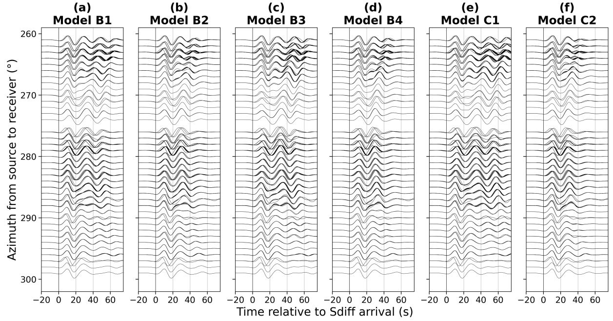
Figure S13. (a-f) Synthetic waveforms for PREM with a cylindrical ULVZ with parameters corresponding to Table S2. Model B & C parameters correspond to off the trade-off curve from the 2DWT inversion ensemble (grey and black circles in Figure S7, respectively). Data are filtered between 10–20 s period.
