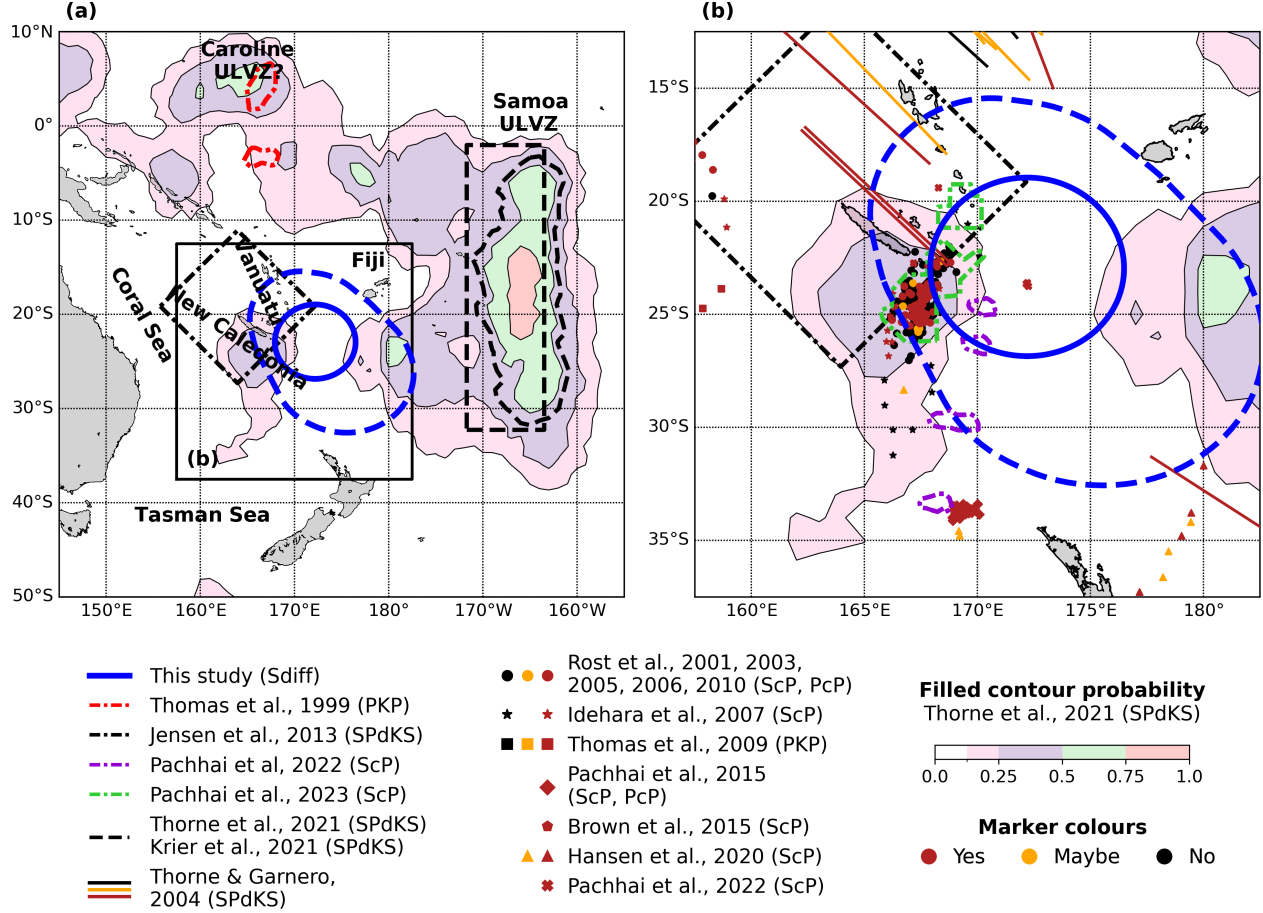
Figure 1. (a) Probability map of the presence of ULVZs based on the 1% misfit map by Thorne et al. [2021]. Note that there is no distinction in this study between low probability and poor data coverage. The dashed black line is the Samoa ULVZ from Thorne et al. [2021] and Krier et al. [2021]. The black dashdotted line gives the proposed ULVZ from Jensen et al. [2013]. The dashed blue line represents the convex hull of our well-fitting parameter space of the ULVZ found in this study. The solid blue line gives the preferred model of the ULVZ in this study, with a radius of 240 km and location 172.2° E and 22.9° S. (b) Zoom-in of the black box in (a) with locations of bounce points on the CMB given by: circles [Rost and Revenaugh, 2001, 2003; Rost et al., 2005, 2006, 2010], stars [Idehara et al., 2007], squares [Thomas et al., 2009], diamonds [Pachhai et al., 2015], pentagons [Brown et al., 2015], triangles [Hansen et al., 2020], and crosses [Pachhai et al., 2022]. The lines are ray paths of SPdKS waveforms on the CMB from Thorne and Garnero [2004]. Their colours indicate the presence (red) and absence (black) of anomalous waveforms; complex waveforms (orange) are not interpreted. The coloured dashdotted lines are proposed ULVZs in the region surrounding Vanuatu from multiple previous studies [Thomas et al., 1999; Thorne et al., 2013; Pachhai et al., 2022, 2023].
