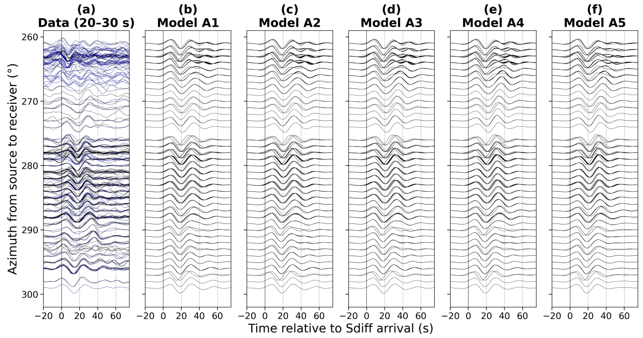
Figure S12. Same as Figure S11 but filtered between 20–30 s period.
