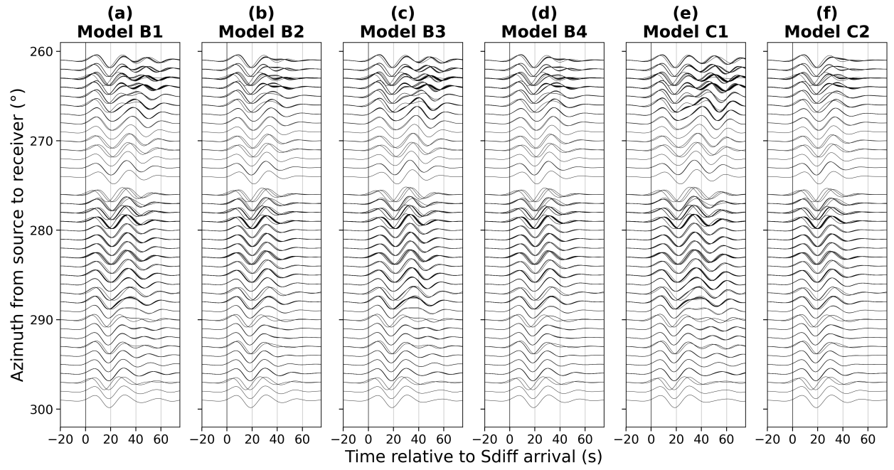
Figure S14. Same as Figure S13 but filtered between 20–30 s period.
