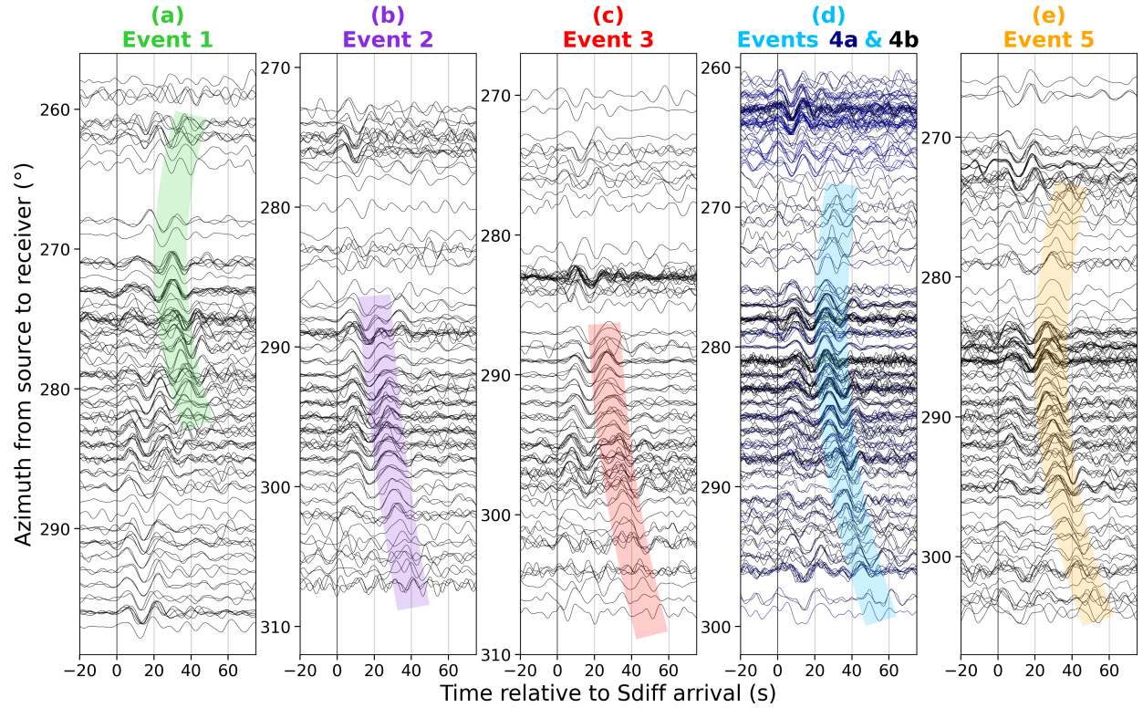
Figure 4. Displacement waveforms on the transverse component filtered between periods of 10–20 s for the six events listed in Table 1. The waveforms are plotted as a function of azimuth (rounded to the nearest integer). The data are plotted with respect to the predicted Sdiff arrival time calculated from the Preliminary Reference Earth Model (PREM, Dziewonski and Anderson [1981]) using the TauP toolkit [Crotwell et al., 1999], adding a constant overall shift for each event up to 10 seconds to shift the reference phase to the predicted arrival time as we expect a shift due to uncertainty in event location and the presence of the LLVP. The shifts applied to each event are included in Table 1. Events 4a (dark blue) & 4b (black) are co-located and plotted together. The Sdiff+ are highlighted, and the colours correspond to the event location stars in Figure 3. Note that the waveforms for Event 2 have been flipped.
