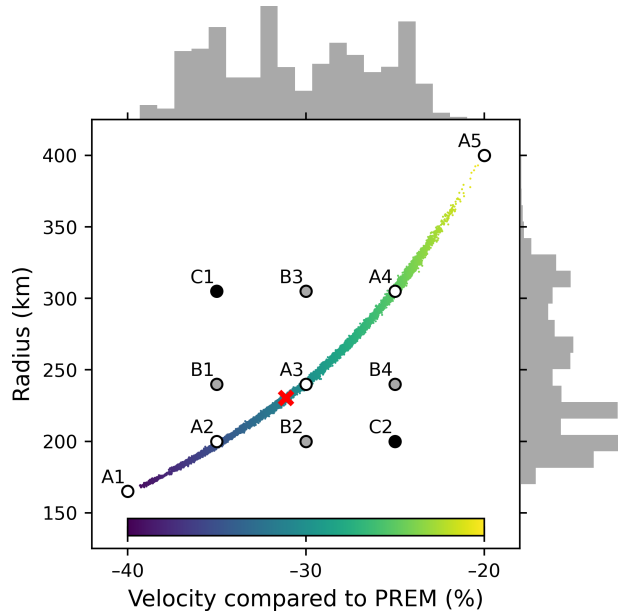
Figure S7. Duplicate of Figure 5b, with parameter labels overlaid. Ensemble of models that fit the Sd-iff postcursor arrival times, showing the trade-off in velocity and size. The median model is marked with a red cross and histograms of each of the parameters are projected onto the respective axes.
