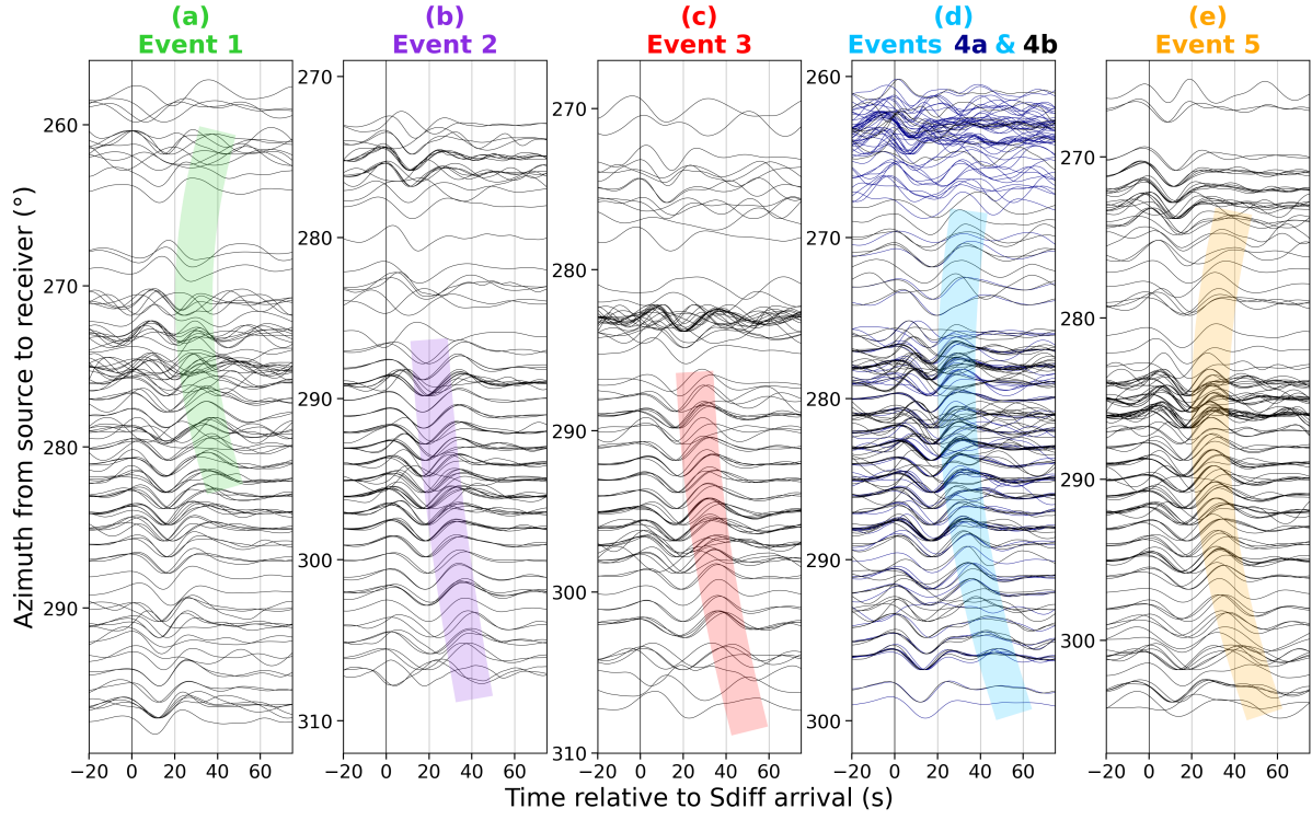
Figure S3. Same as Figure 4 but filtered between 30–40 s period.
