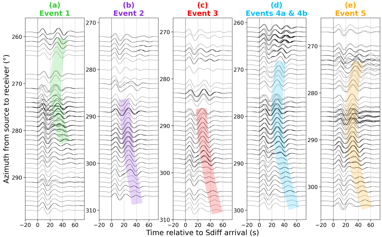
Figure 6. Displacement synthetics for PREM with a ULVZ with height 20 km, radius 240 km, and shear velocity reduction of 30% (Model A3, Table S2) filtered between periods of 10–20 s for the six events listed in Table 1. The same Sdiff+ highlights from Figure 4 are overlaid, and the colours correspond to the event location stars in Figure 3.
