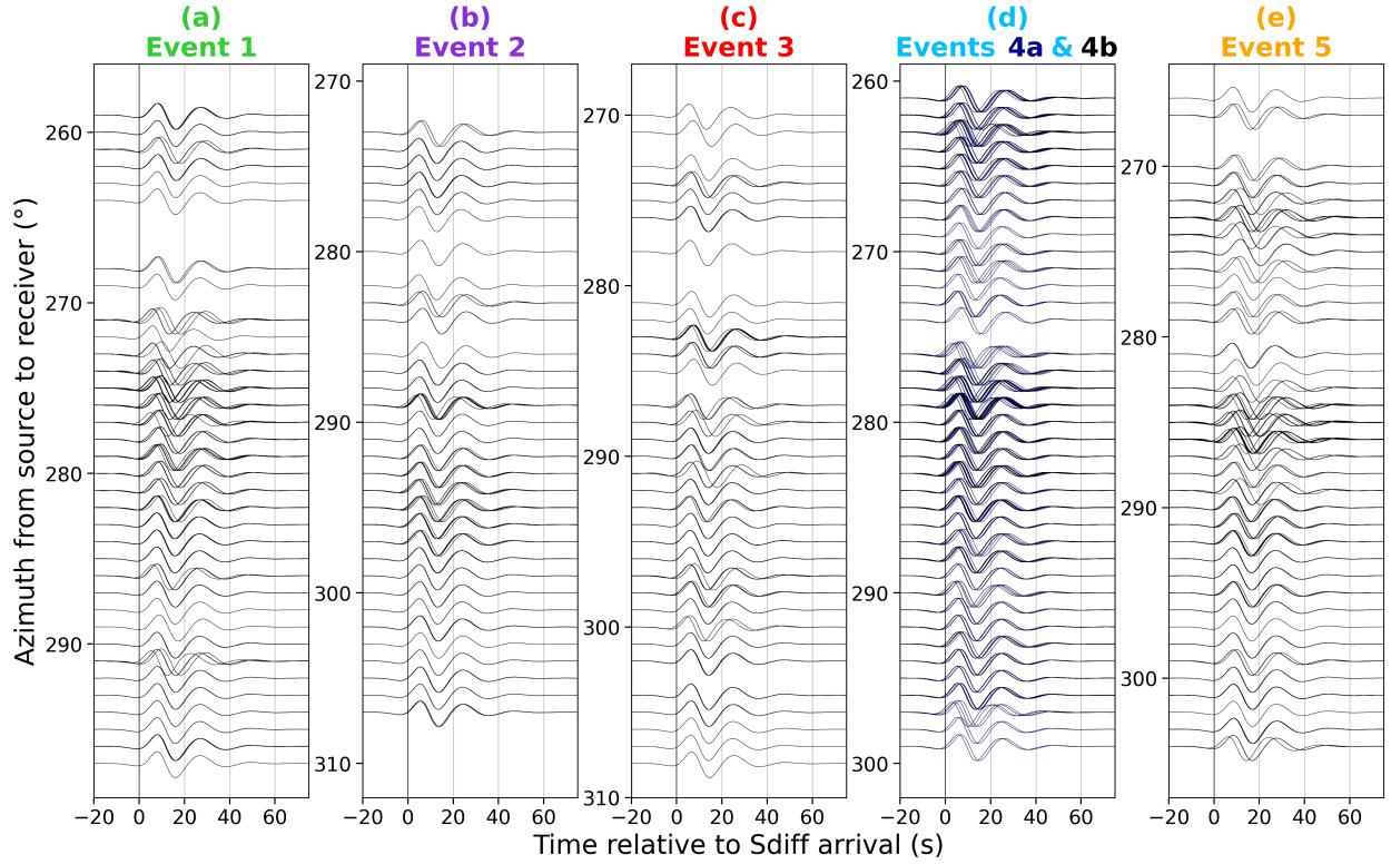
Figure S6. Displacement synthetics for PREM filtered between periods of 10–20 s for the six events listed in Table 1. Earthquake parameters and moment tensor solutions are taken from the Global CMT Project [Ekström et al., 2012], with depths set to 0 km.
