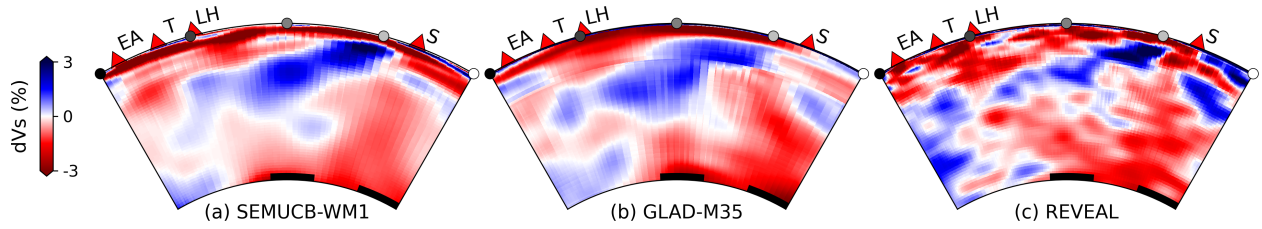
Figure 8. Cross-sections of recent whole mantle tomographic models (a) SEMUCB-WM1 [French and Romanowicz, 2014], (b) GLAD-M35 [Cui et al., 2024], and (c) REVEAL [Thrustarson et al., 2024] through the transect on Figure 3, which passes through the Vanuatu and Samoa ULVZs and near the Lord Howe and Samoa hotspots. Velocity deviations are with respect to the (whole Earth) radial average of each tomographic model. Nearby hotspots are projected onto the cross-section: EA = East Australia, T = Tasmantid, LH = Lord Howe, and S = Samoa. ULVZ thickness (solid black lines) is exaggerated for visualisation.
