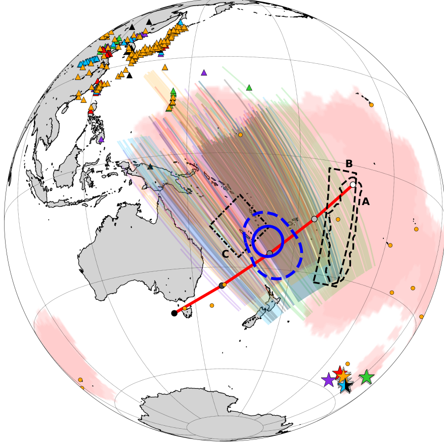
Figure 3. Map of event locations (stars), receivers (triangles) and the Sdiff ray paths sensitive to the CMB (below 2800 km depth). The earthquakes and ray paths are coloured per event: 1–green, 2–purple, 3–red, 4a–blue, 4b–black and 5–orange (Table 1); light grey stars are events identified but not analysed (Table S1). Hotspot locations are shown as orange circles. The dashed blue line represents the convex hull of ensemble of models of ULVZs which fit the Sdiff+ arrival time data in this study. The solid blue line gives the preferred model of the ULVZ in this study, with a radius of 240 km and location 172.2° E and 22.9° S. The models of the Samoa ULVZ are given as black dashed lines: A–irregular shaped [Thorne et al., 2021] and B–rectangular shaped [Krier et al., 2021]. The black dashdotted line shows the inferred C–diamond shaped ULVZ from Jensen et al. [2013]. The background displays the LLVP vote map at 2800 km depth [Cottaar and Lekic, 2016]. The solid red line and greyscale markers denote the cross-section transect in Figure 8.
