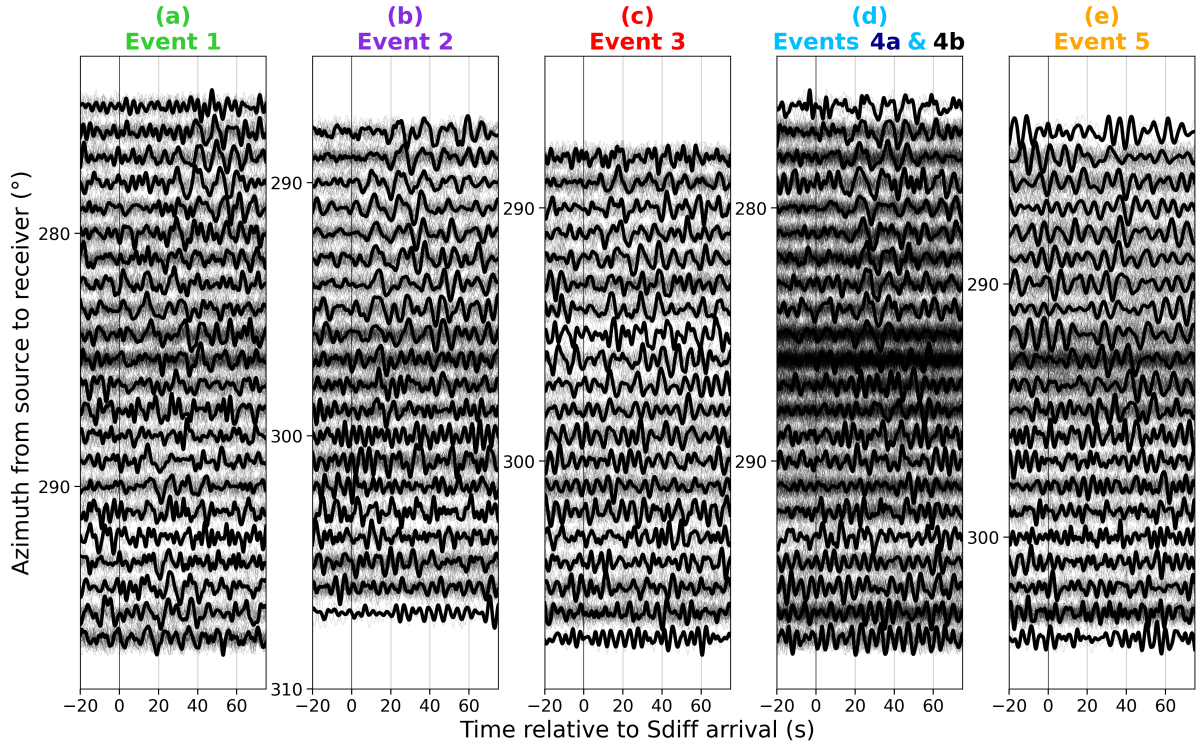
Figure S5. Same as Figure S4 but filtered between 7–12 s period.
