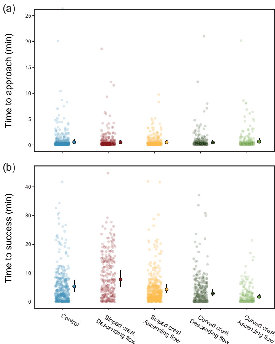
FIGURE 6 Actual and predicted median transit time (in minutes) of Anguilla anguilla on eel pass trials. From (a) the approach to the crest and (b) the first point of contact with the crest to successfully completing the pass for each treatment and the control. Point estimates represent posterior medians, whereas error bars denote 95% credible intervals (CIs). Raw data are displayed with small, open circles. The cartesian coordinates of the plots were restricted to exclude five outliers in plot (a) and 12 outliers in plot (b). This was done to better visualise treatment-level differences in median transit time. However, these outliers were included in all models and are accounted for in model estimated posterior medians and CIs that are displayed on the plots.
