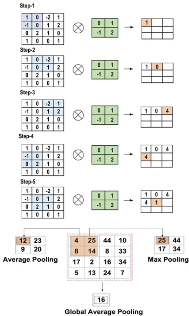
Fig. 3. Procedure and filters for CNN model.
