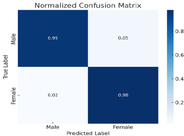
Fig. 5. Confusion matrix for the deployed model.
