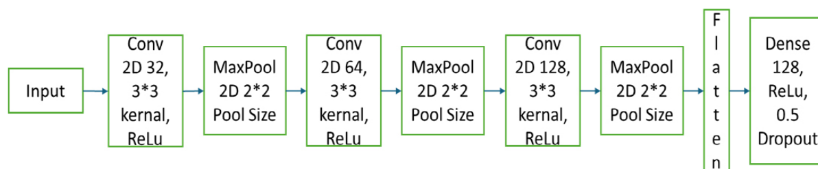
Fig. 2. Architecture of the proposed model.
