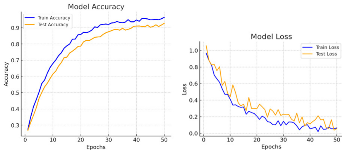
Fig. 4. Plots of accuracy and loss of employed model.
