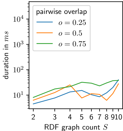
RDF graph size n = 100
