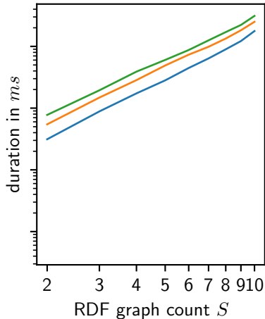
RDF graph size n = 100000
