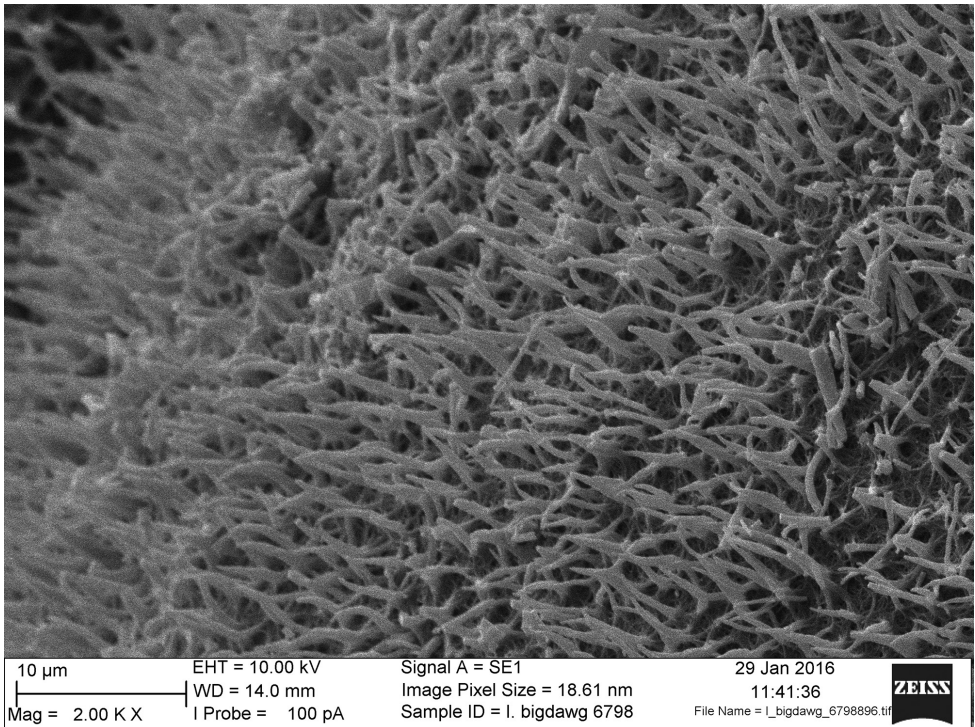
Figure 2. SEM detail of megaspore micro-ornamentation. Magnification 2000x.
