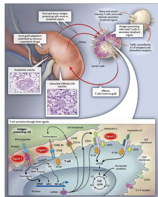
Figure 2: 3 signal model [8] is widely recognised as the steps in rejection in allo-immune responses.
