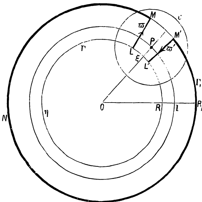
The contribution of \Sigma_{p,q}^1 .
