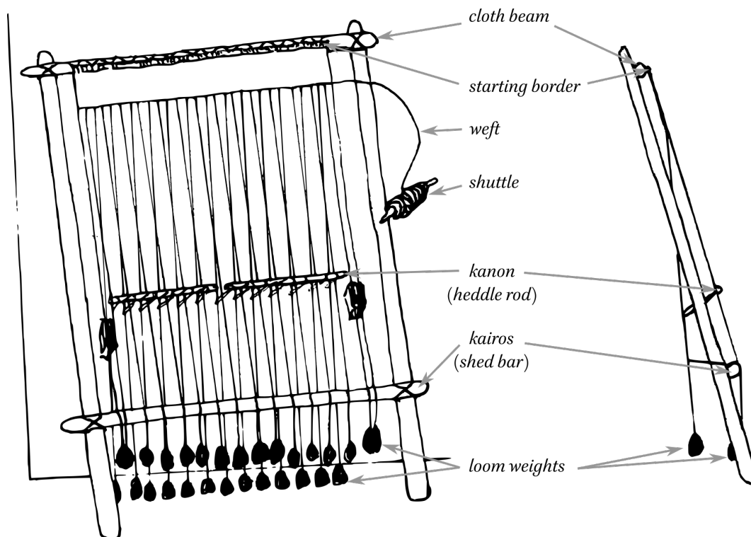
FIGURE 2. THE COMPONENTS OF A WARP-WEIGHTED LOOM, AS USED IN ANCIENT GREECE.
