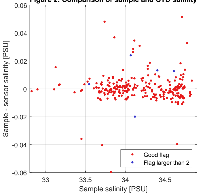
Figure 2: Comparison of sample and CTD salinity
