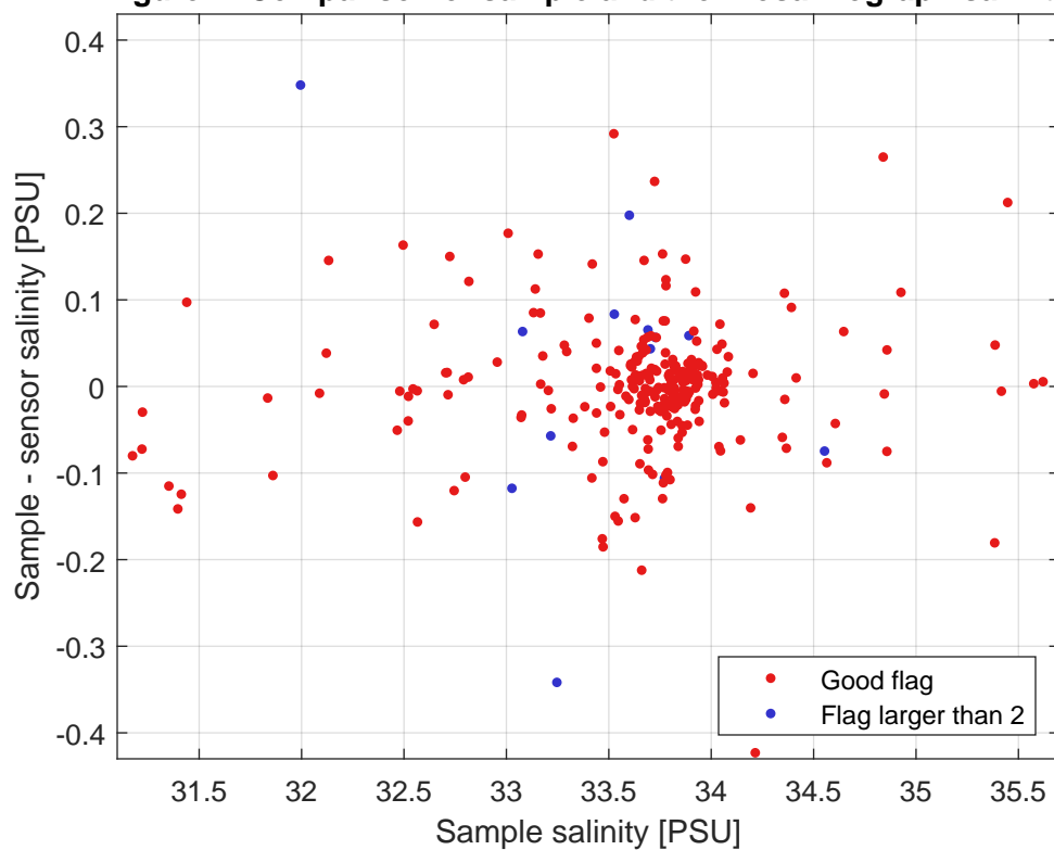
Figure 1: Comparison of sample and thermosalinograph salinity
