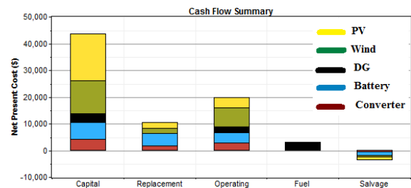
Fig. 8. Cash flow summary based on cost.
