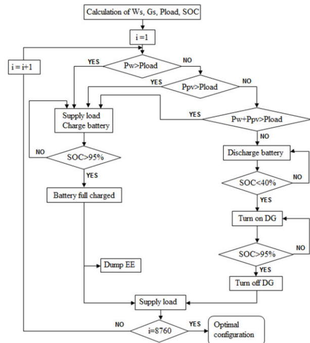
Fig. 4. Flow chart of energy management.
