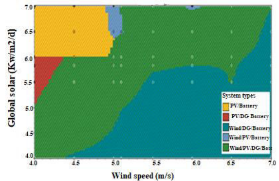
Fig. 10. Optimal system for fixed diesel price and hub height.
