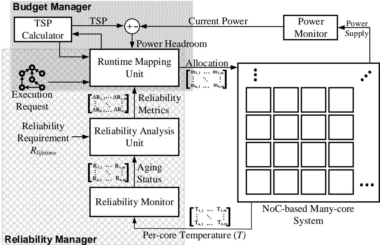
Figure 4. High-level architecture implementing throughput-driven vs. reliability-driven mapping strategy
