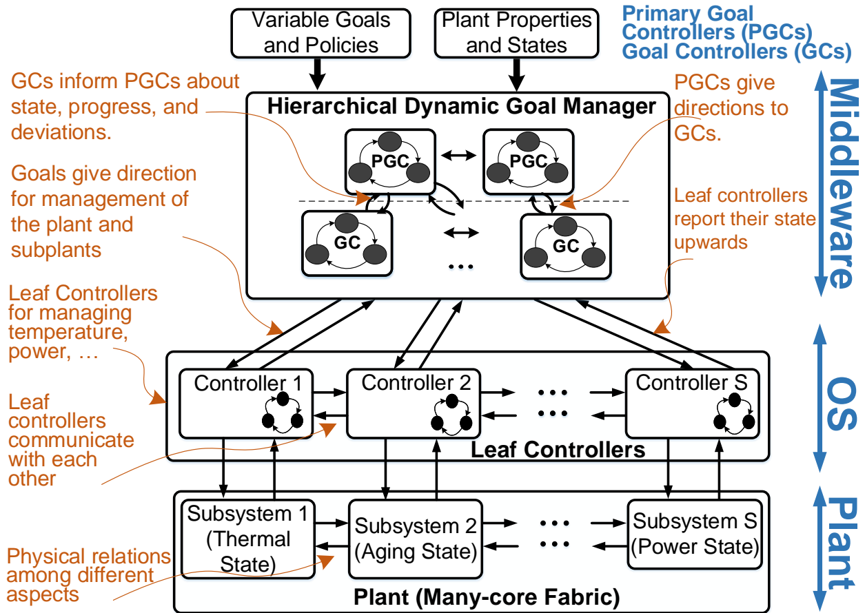
Figure 6. High-Level architecture for hierarchical dynamic goal management.
