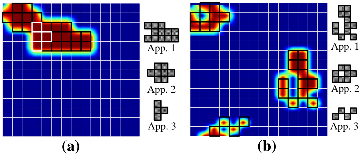
Figure 3. Effect of mapping on temperature accumulation [10]
