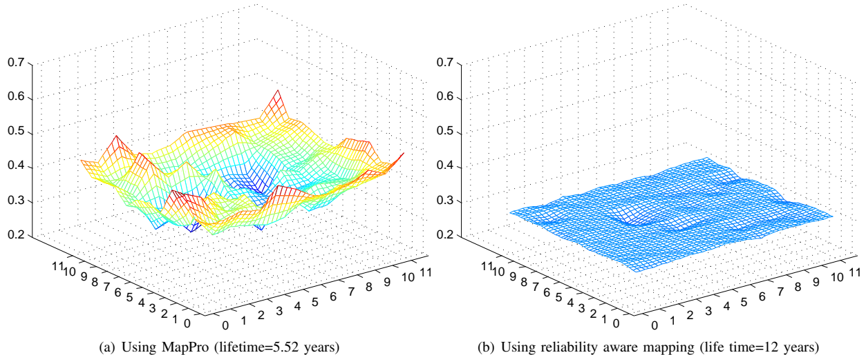
Figure 5. The effect of different runtime mapping approached on overall system lifetime (until the first core's reliability reaches 30%) [9]
