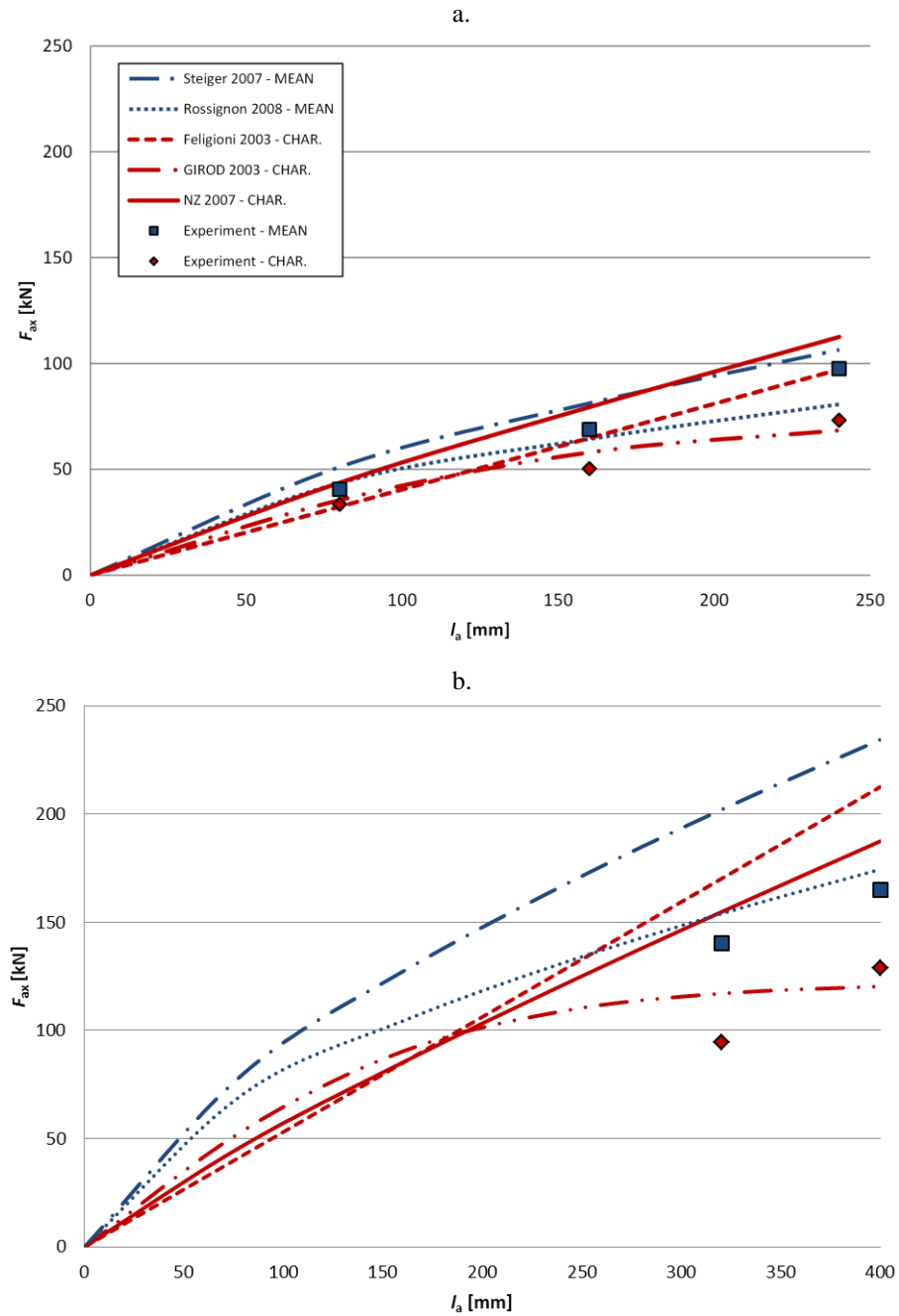
Fig. 6 Comparison of pull-out strength equations with experimental data for the 0° specimens: a.) d_h = 20 mm, and b.) d_h = 28 mm
