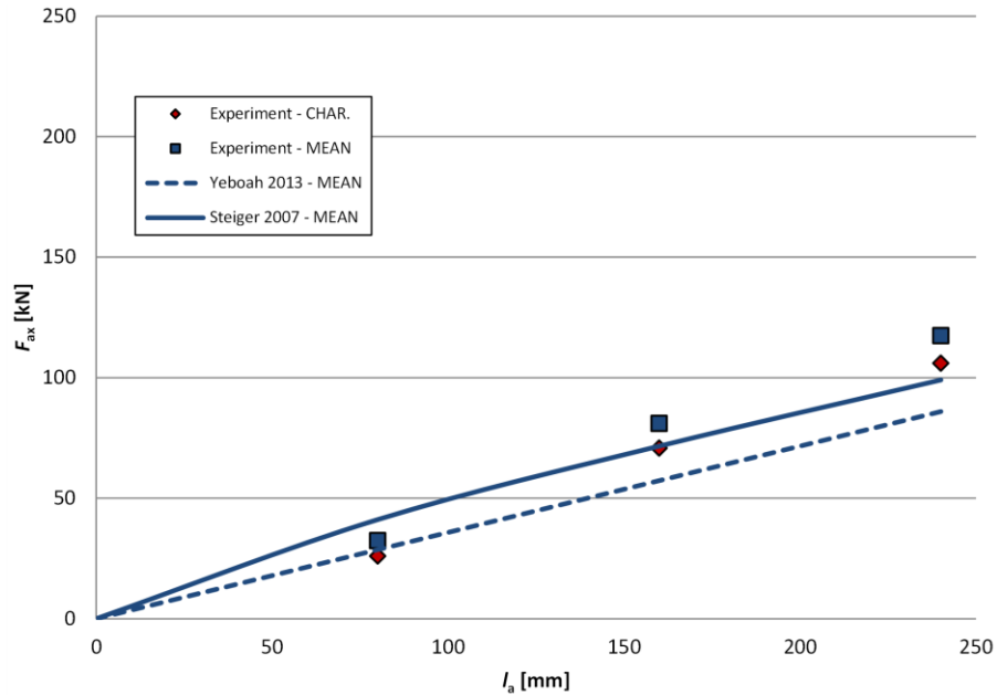
Fig. 7 Comparison of pull-out strength equations with experimental data for the 90^\circ specimens
