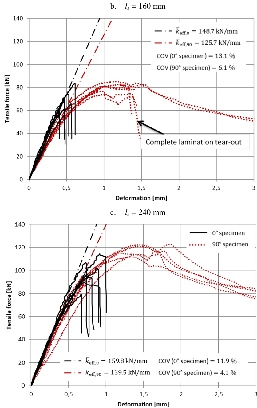
Fig. 3 Results for specimens with: a.) l_a = 80 mm, b.) l_a = 160 mm and c.) l_a = 240 mm
