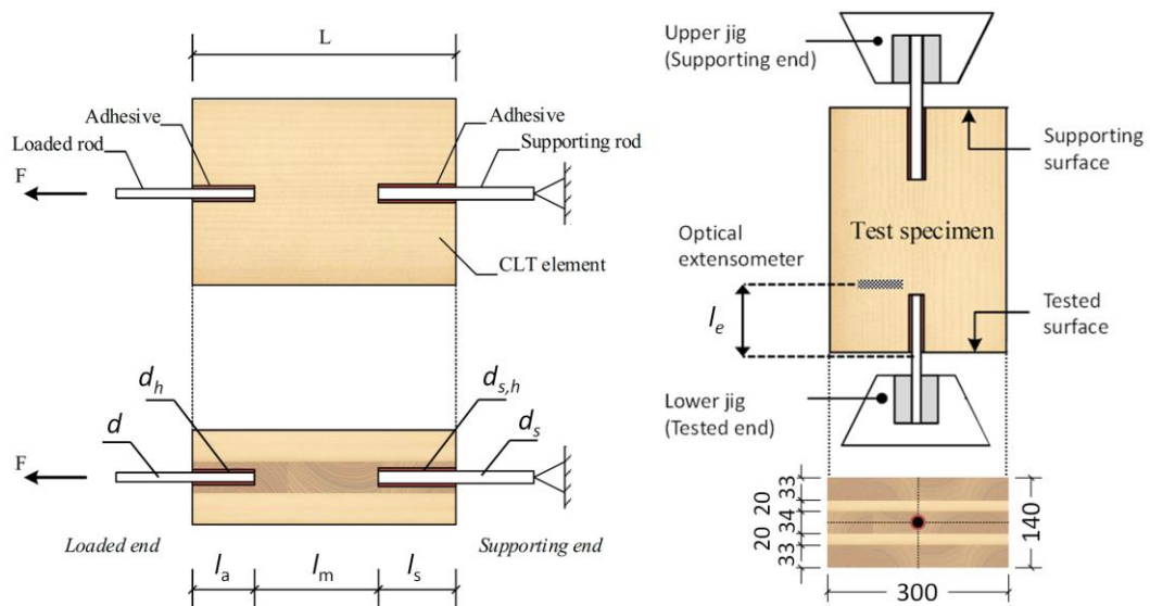
Fig. 1 Test specimen and test set-up [19]
