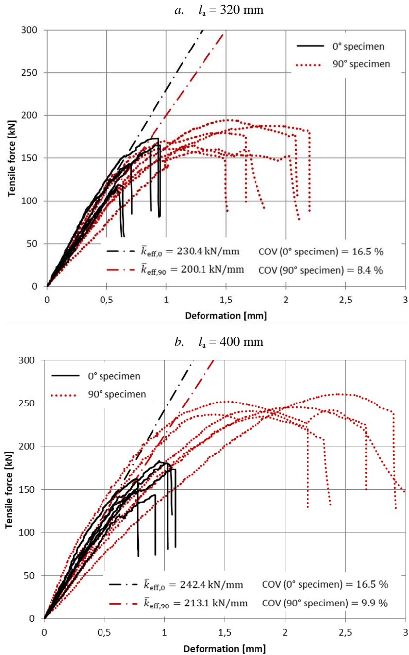
Fig. 5 Results for specimens with: a.) l_a = 320 mm and b.) l_a = 400 mm
