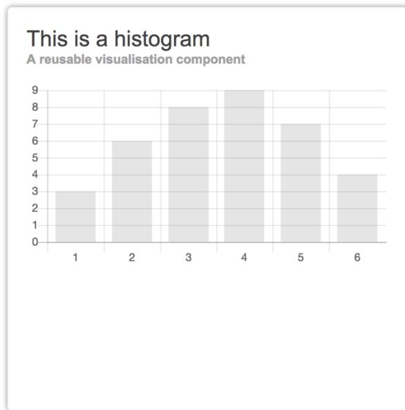
Figure 3. Histogram
