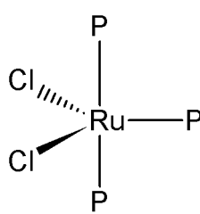
equatorial
