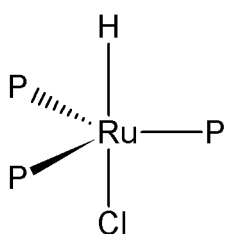
axial,trans
