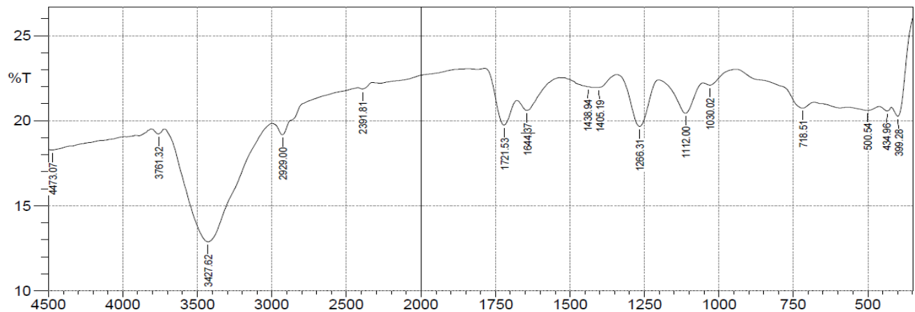
Fig. 2: FT-IR of P. thonningii flower extract (X and Y axes are wavenumber (cm -1 ) and % Transmittance respectively)
