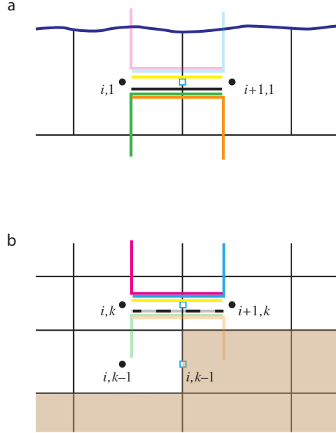
FIGURE E.3: (a) Uppermost model layer k = 1 with i, 1 and i + 1, 1 tracer points (black dots), and i + 1/2, 1 u -point (blue square). Triad slopes \frac{1}{i} \mathbb{R}_{1/2}^{-1/2} (magenta) and \frac{1}{i+1} \mathbb{R}_{-1/2}^{-1/2} (blue) poking through the ocean surface are masked (faded in figure). However, the lateral _{11} contributions towards \frac{1}{i} \mathbb{F}_{u_{1/2}}^{-1/2} and \frac{1}{i+1} \mathbb{F}_{u_{-1/2}}^{-1/2} (yellow line) are still applied, giving diapycnal diffusive fluxes. (b) Both near bottom triad slopes \frac{k}{i} \mathbb{R}_{1/2}^{1/2} and \frac{k}{i+1} \mathbb{R}_{-1/2}^{1/2} are masked when either of the i, k + 1 or i + 1, k + 1 tracer points is masked, i.e. the i, k + 1 u -point is masked. The associated lateral fluxes (grey-black dashed line) are masked if botmix_grif=false. , but left unmasked, giving bottom mixing, if botmix_grif=true.
