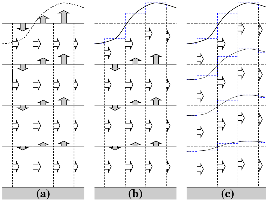
FIGURE 2.3: (a) z -coordinate in linear free-surface case; (b) z -coordinate in non-linear free surface case; (c) re-scaled height coordinate (become popular as the z^* -coordinate [Adcroft and Campin 2004] ).
