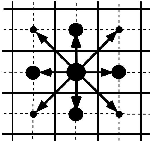
FIGURE 9.1: averaging procedure for isopycnal slope computation.
