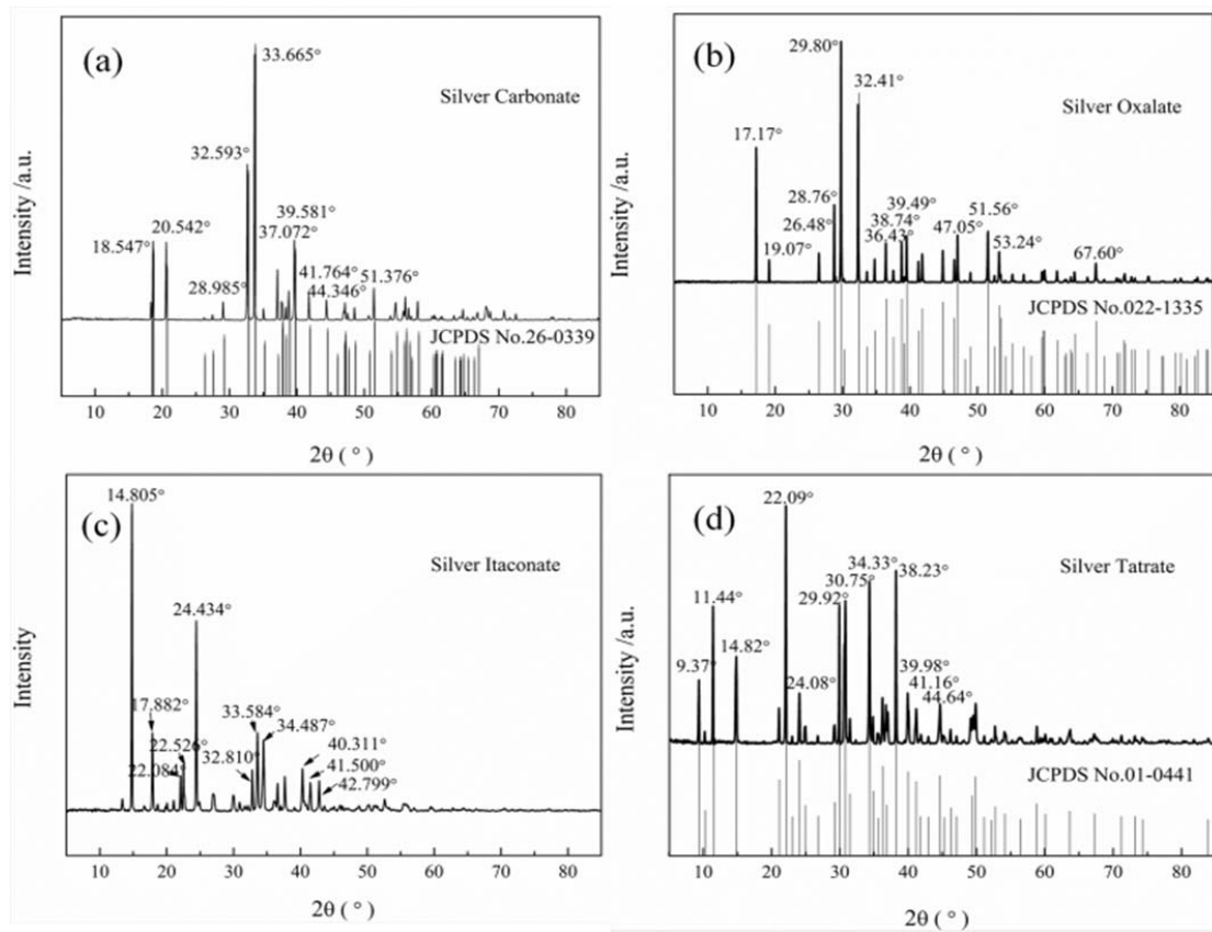
Fig. 2 XRD patterns of four as-prepared silver carboxylates
