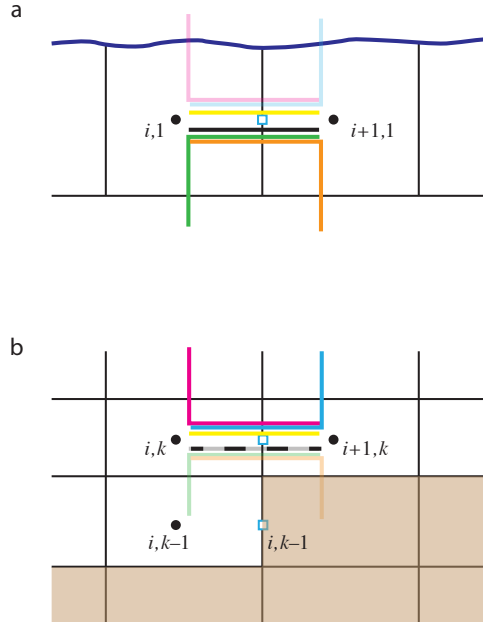
Figure D.3: (a) Uppermost model layer k = 1 with i, 1 and i + 1, 1 tracer points (black dots), and i + 1/2, 1 u -point (blue square). Triad slopes ^1_i\mathbb{R}_{1/2}^{-1/2} (magenta) and ^1_{i+1}\mathbb{R}_{-1/2}^{-1/2} (blue) poking through the ocean surface are masked (faded in figure). However, the lateral _{11} contributions towards ^1_i\mathbb{F}_{u_{1/2}}^{-1/2} and ^1_{i+1}\mathbb{F}_{u_{-1/2}}^{-1/2} (yellow line) are still applied, giving diapycnal diffusive fluxes. (b) Both near bottom triad slopes ^k_i\mathbb{R}_{1/2}^{1/2} and ^k_{i+1}\mathbb{R}_{-1/2}^{1/2} are masked when either of the i, k + 1 or i + 1, k + 1 tracer points is masked, i.e. the i, k + 1 u -point is masked. The associated lateral fluxes (grey-black dashed line) are masked if botmix_grif =false., but left unmasked, giving bottom mixing, if botmix_grif =true.
