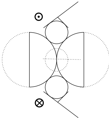
Fig. 34: The spherical balls
