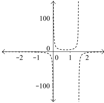
Fig. 9: v(t) function for x : 1 and y : 50 scale
