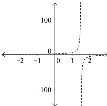
Fig. 10: x(t) function for x : 1 and y : 50 scale
