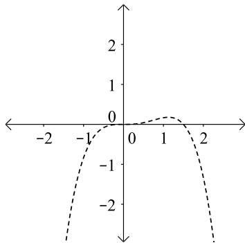
Fig. 6: A/\Delta a function
