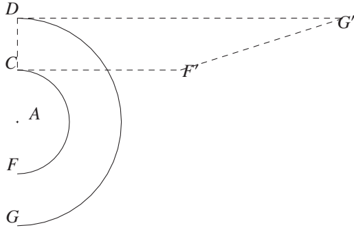
Fig. 32: The area of the circle in the kind of triangle
