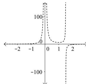
Fig. 8: a(t) function for x : 1 and y : 50 scale
