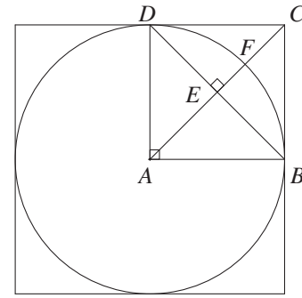
Fig. 29: Internal tangent circle
