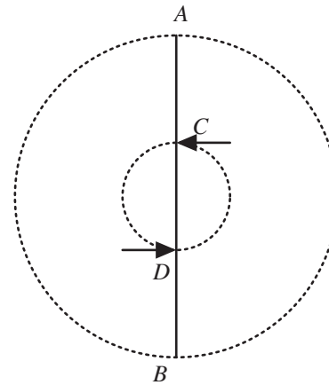
Fig. 35: An object which is about to go at light speed
