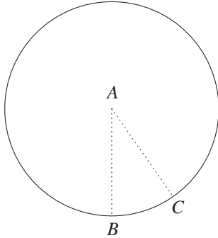
Fig. 25: Two points on the circumference
