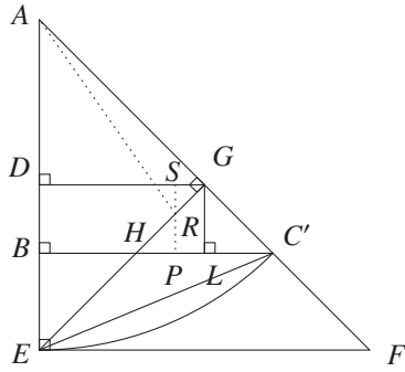
Fig. 28: A part of Fig. 27
