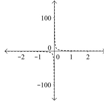
Fig. 7: f(t) function for x : 1 and y : 50 scale
