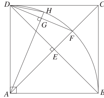
Fig. 30: The quarter slice of Fig. 29
