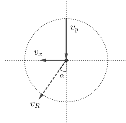
Fig. 21: The resultant movement
