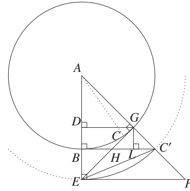
Fig. 27: The second radius
