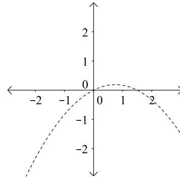
Fig. 4: A/\Delta x function
