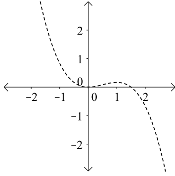
Fig. 5: A/\Delta v function
