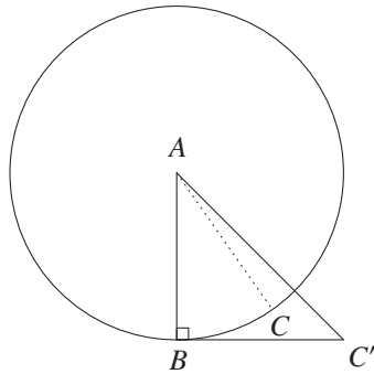
Fig. 26: The arc side
