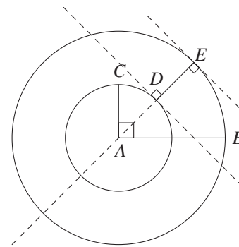
Fig. 31: The area scanned
