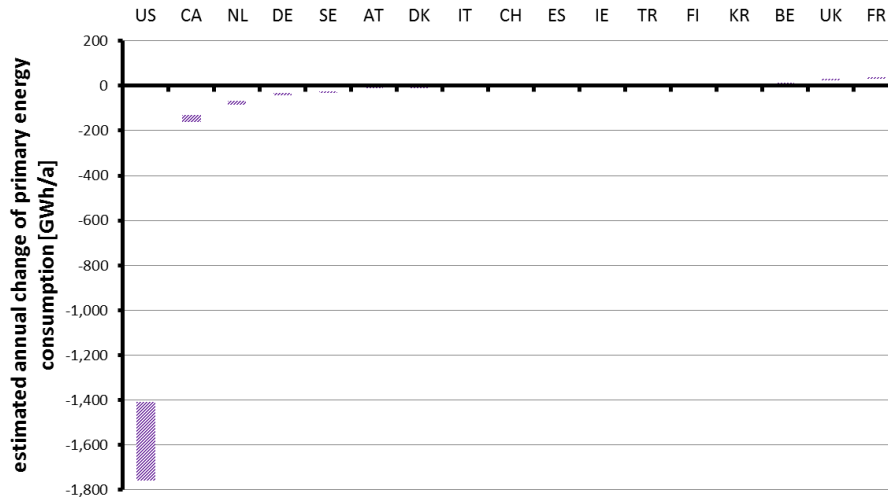
Fig. 9: Estimated range of annual primary energy changing of 0.8 Mio EVs substituting ICE vehicles in IEA HEV countries in 2015
