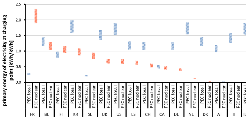
Fig. 5: Estimated range of cumulated fossil and nuclear primary energy for electricity generation at charging point in IEA HEV countries in 2015
