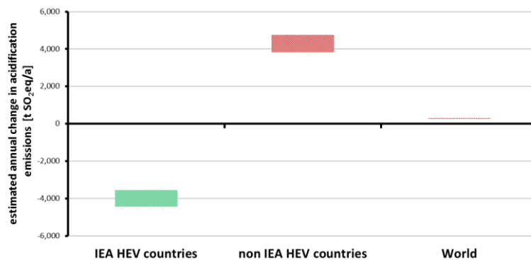
Fig. 11: Estimated range of change in acidification of 1.3 Mio. EVs substituting ICE vehicles globally in 2015
