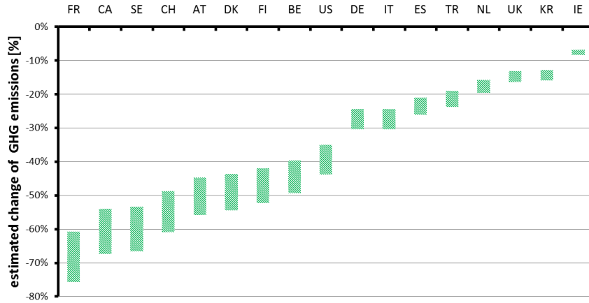
Fig. 6: Estimated range of GHG emissions reduction of EVs substituting ICE vehicles in IEA HEV countries in 2015
