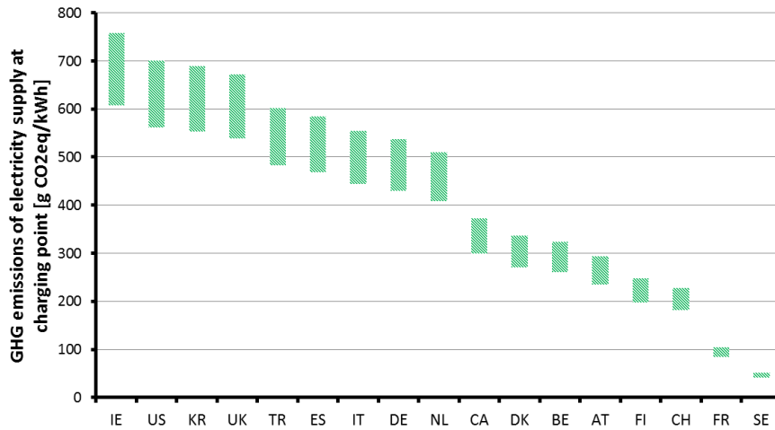
Fig. 4: Estimated range of GHG emissions of electricity at charging point in IEA HEV countries in 2015
