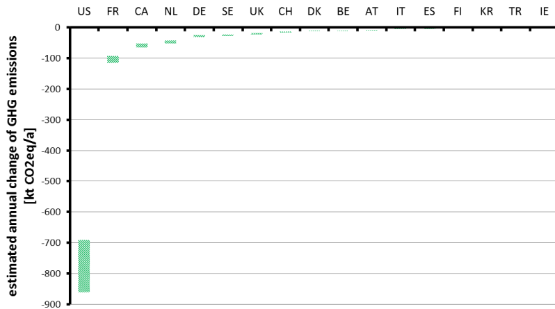
Fig. 8: Estimated range of annual GHG emissions reduction of 0.8 Mio EVs substituting ICE vehicles in IEA HEV countries in 2015
