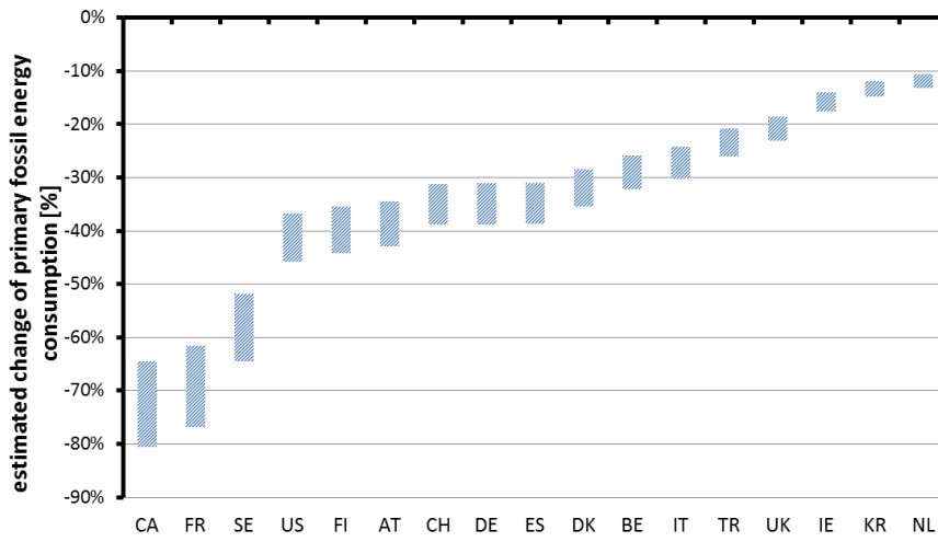
Fig. 7: Estimated range of fossil primary energy reduction of EVs substituting ICE vehicles in IEA HEV countries in 2015
