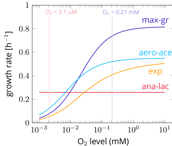
Figure 7.6: Monod curves (cell growth rate as a function of oxygen level) computed using the model shown in Figure 7.5 – Each curve was computed using one of the EFMs and the associated (oxygen-dependent) enzyme demands. The ana-lac strategy (anaerobic growth with lactate secretion) does not use oxygen, therefore its curve is flat.
