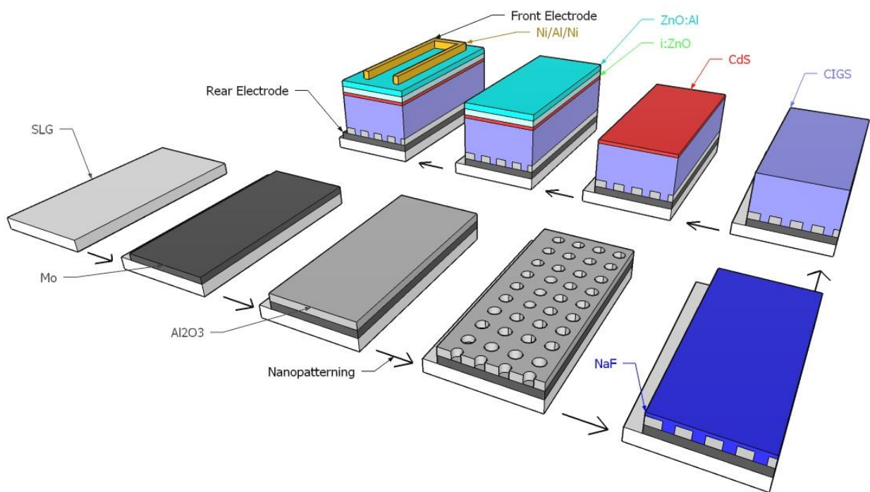
Figure 1: representation of the solar cell fabrication process of the passivation sample. The reference device excluded the \text{Al}_2\text{O}_3 deposition and the nanopatterning steps.
