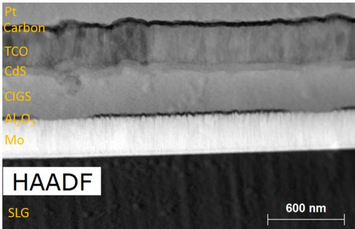
Figure 2: TEM HAADF image of the cross-section of the passivated solar cell. The dark layer in-between the Mo layer and the CIGS layer, is the \text{Al}_2\text{O}_3 passivation layer. The observed openings on this \text{Al}_2\text{O}_3 layer are the nanopatterned point contacts.
