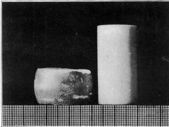
Column of marble before and after compression under a load of 296,725 pounds per square inch (20,875 kilos. per square cent.). The finer lines of the scale are one millimeter apart.
