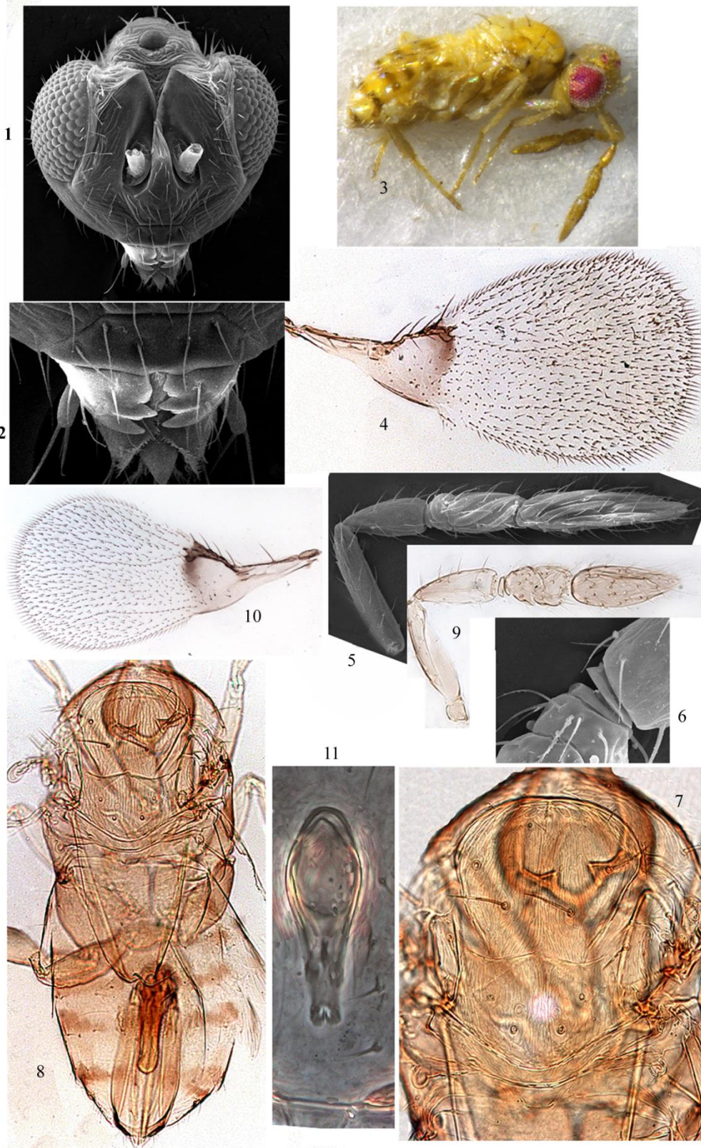
FIGURES (1-11). Chaetogramma hisarensis , female: 1, head; 2, mandible; 3, habitus; 4, fore wing; 5, antenna; 6, anelli; 7, mesosoma; 8, body. male: 9, antenna; 10, fore wing; 11, phallus.
