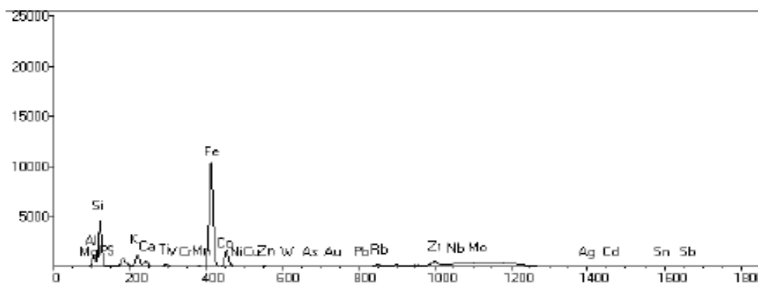
Figure 2: XRF analysis result for Ara-Ekiti Clay
