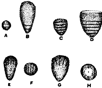
FIG. 3.—A, basidiocarp marked with India ink when 3 mm. high to determine region of growth; B, same 10 mm. high; C, basidiocarp marked when 5 mm. high; D, position of marks at time of expansion; E, F, side and end views of basidiocarp marked just before expansion; G, H, same basidiocarp with peridium breaking away and epiphragm showing in center.
