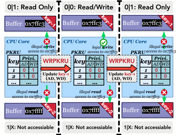
Figure 6: An example of switching the access privileges of MPK keys via WRPKRU. The memory page 0x7ffc3 is tagged with key-1 . The memory page 0x7fff is tagged with key-2 .
