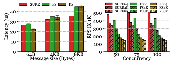
Figure 12: Performance of SURE’s Z-stack: (left) latency with 1 connection; (right) RPS under different concurrency levels. FS: F-stack; KS: kernel stack.
