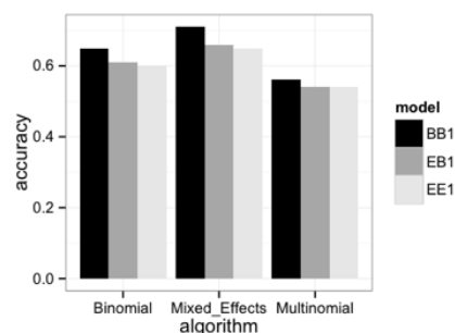
Figure 5: Model accuracy overview: binomial, mixed-effects, multinomial models
