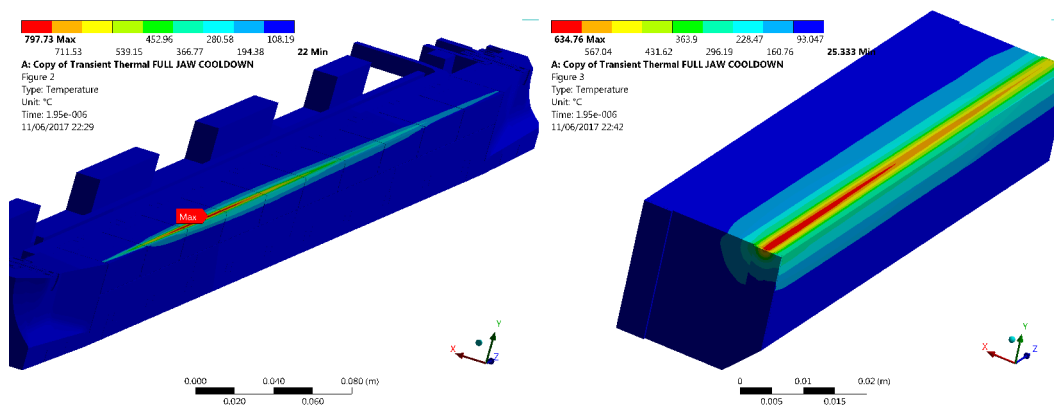
Figure 111. Left: temperature distribution after impact #32 on the CuCD jaw. The peak is found on the 3 rd CuCD block. The model presents a symmetry along the section plane parallel to XZ . Right: temperature distribution on the 5 th CuCD block ( z = 400 \div 500 mm).
