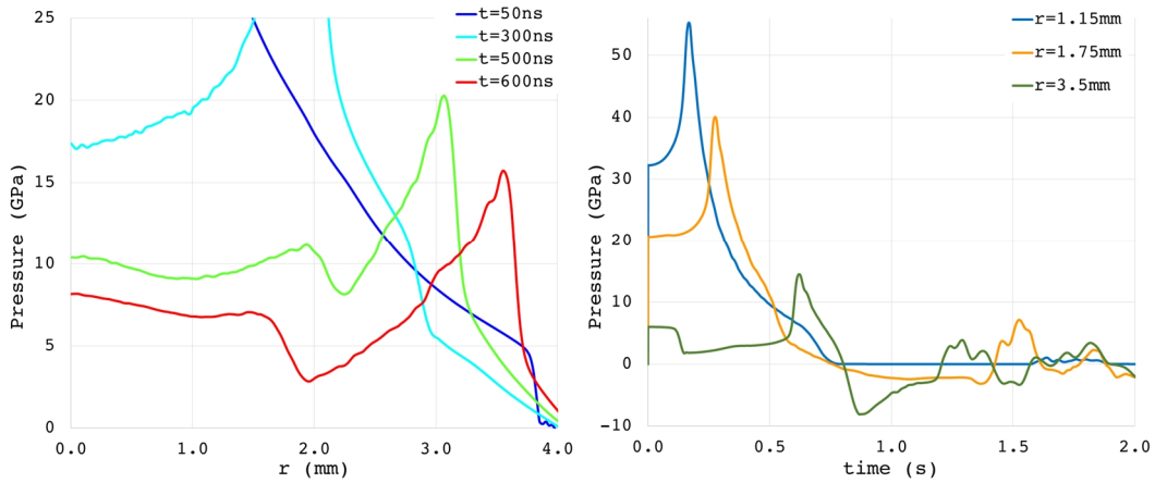
Figure 64. Left: pressure wave along the radius, for z=220\text{mm} , at different time instants. Right: pressure during time on three elements with z=220\text{mm} and different radial coordinate.
