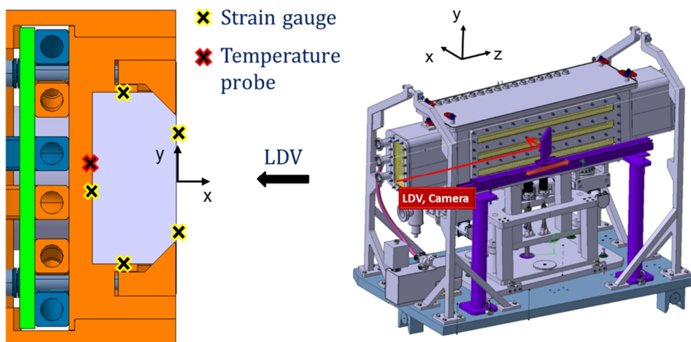
Figure 92. Left: HL-LHC jaw section, strain gauge and temperature probe configuration. Right: movable mirror for laser-Doppler vibrometer and HD camera acquisition.
