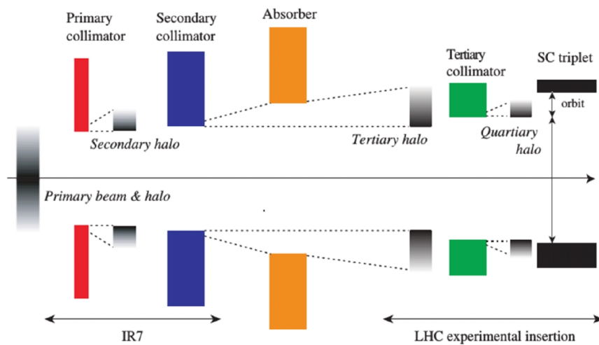
Figure 74. Scheme of the LHC collimation system, courtesy of E. Quaranta.
