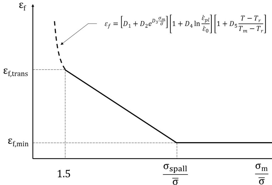
Figure 36. Johnson-Cook failure model, definition of fracture strain at large tensile pressure-stress ratios.
