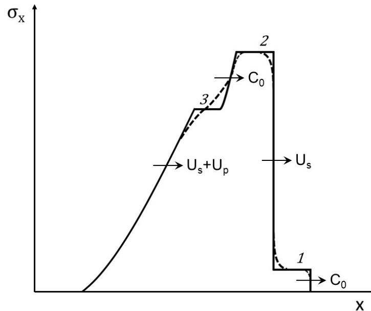
Figure 31. Elastoplastic material, shock wave and release.
