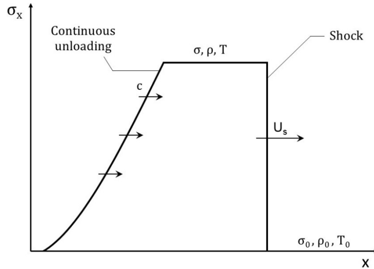
Figure 27. Idealized shock profile.
