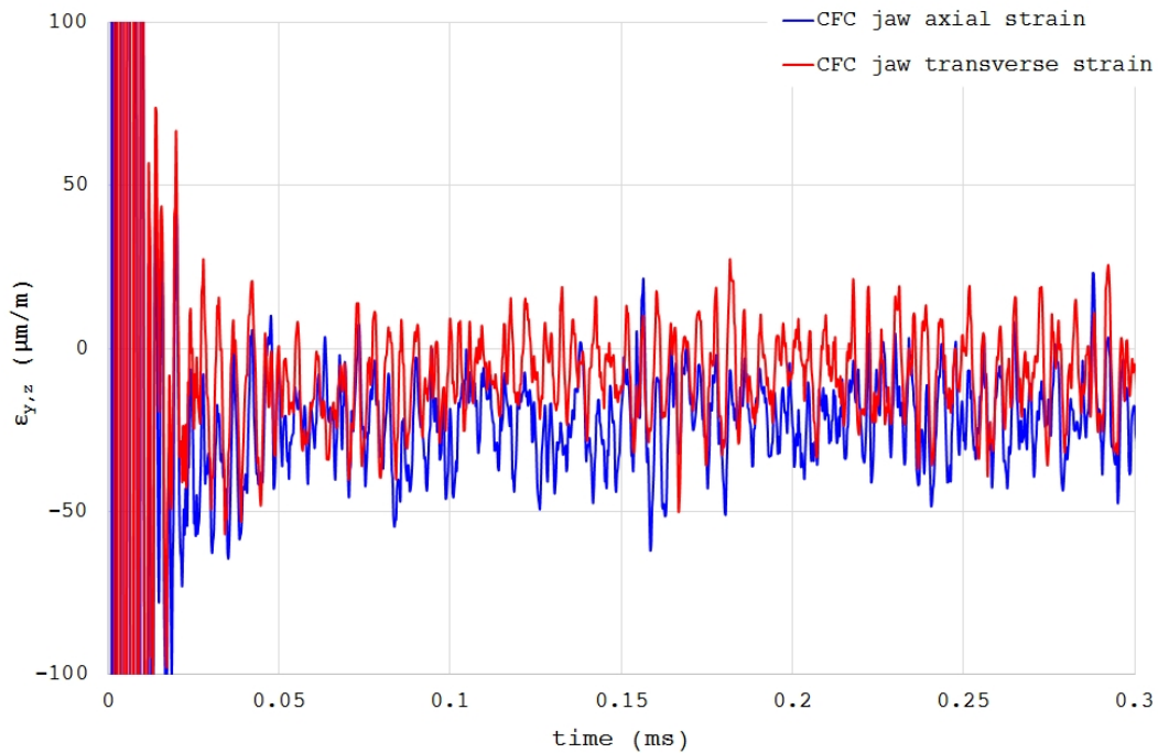
Figure 129. Impact #7 , CFC: experimental transverse and axial strain on the back face of the jaw, at a longitudinal coordinate z = 780 mm.
