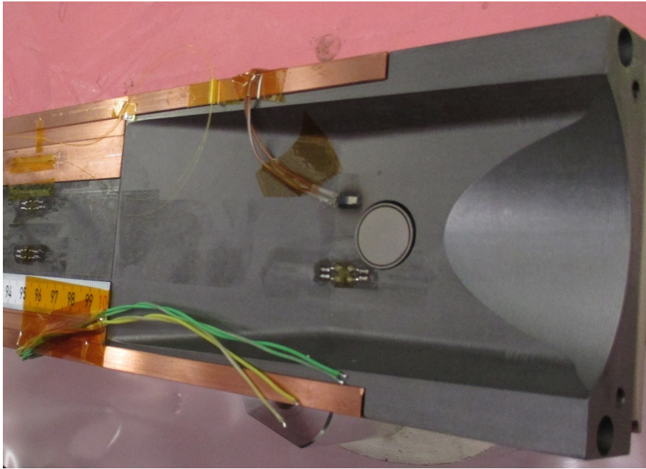
Figure 98. View of the downstream MoGr tapering. No sign of damage to the component or to the BPM is evident.
