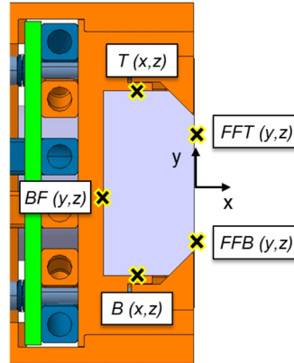
Figure 109. Strain gauge positioning and nomenclature, with the acquired strain direction in each point under parenthesis. T is the top face, B the bottom face, BF the back face, FFT and FFB the front face top and bottom gauges.
