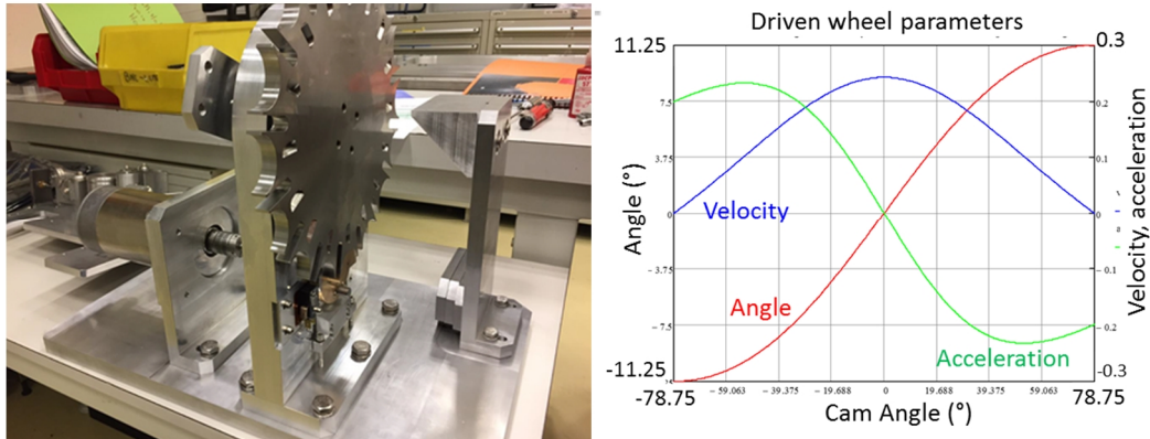
Figure 136. Left: mock-up of the Geneva mechanism. Right: driven wheel parameters as function of the cam angle.
