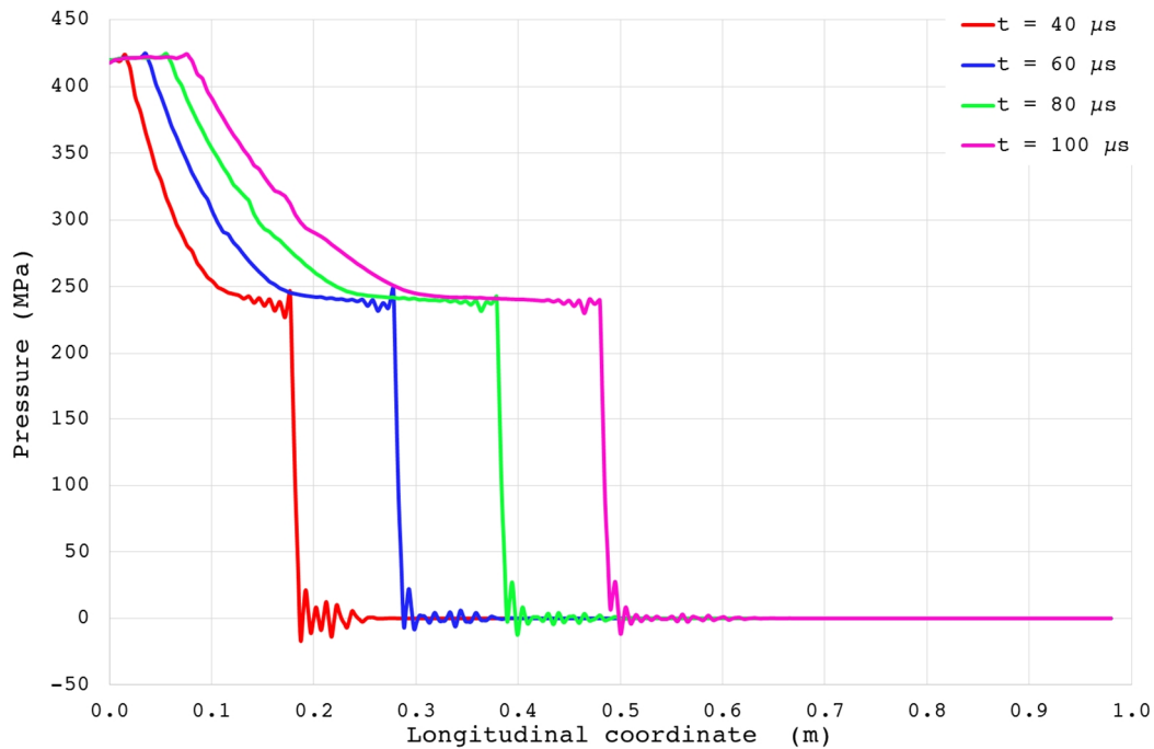
Figure 16. Wave front on a 2024 aluminum cylinder at given time instants. Note the constant velocity of propagation of the elastic front up to the yield stress. In the plastic domain, the velocity decreases with the increase of stress.
