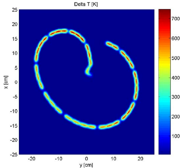
Figure 5. Temperature distribution on the LHC dump [16]. Note the spiral pattern dilution.
