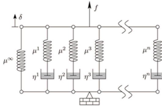
Figure 32. Generalized Maxwell solid in one dimension, adopted for the definition of uniaxial viscoelastic models in ANSYS [17]. The spring stiffnesses are \mu^i , the dashpot viscosities are \eta^i , and the relaxation time is defined as the ratio of viscosity to stiffness, \tau^i = \eta^i / \mu^i .
