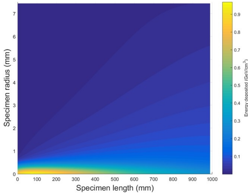
Figure 37. Energy density generated by a proton beam impact on a graphite target rod, L = 1 m, \varnothing = 15 mm, courtesy of M. I. Frankl. The beam energy is 440 GeV and the \sigma is 0.25 mm. The specific energy is normalized to one proton.
