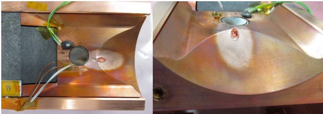
Figure 96. Views of the damage on the downstream Glidcop tapering of the CFC jaw. The high temperatures generated by the impact are also highlighted by the oxidation of the Glidcop surface and of the BPM button.
