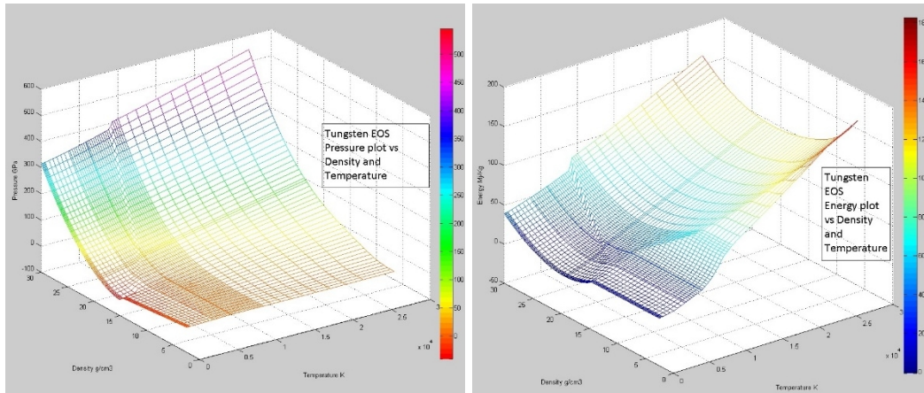
Figure 26. SESAME table 3550, built for tungsten. Left: pressure as a function of density and temperature. Right: Energy as a function of density and temperature.
