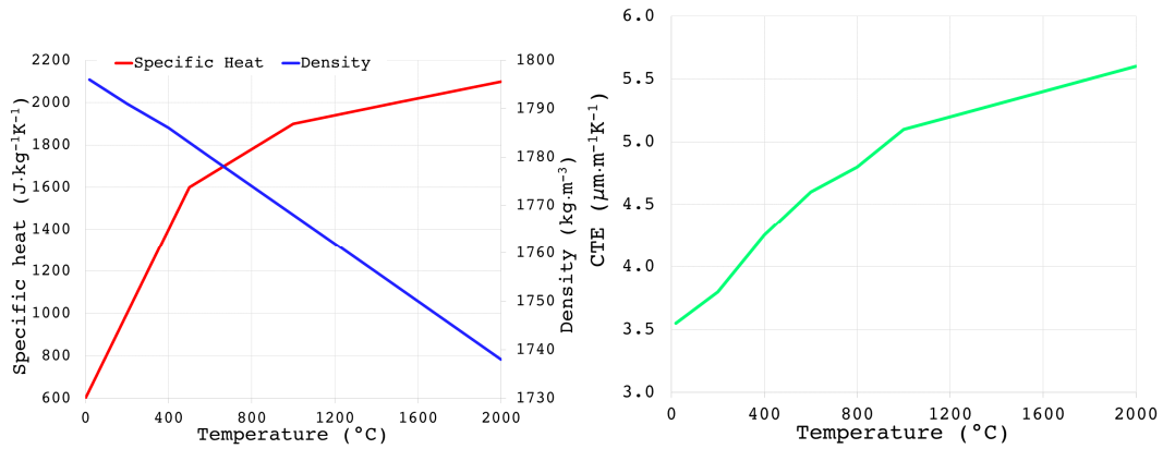
Figure 45. Left: specific heat and density of isostatic graphite as a function of temperature. Right: coefficient of thermal expansion as a function of temperature.
