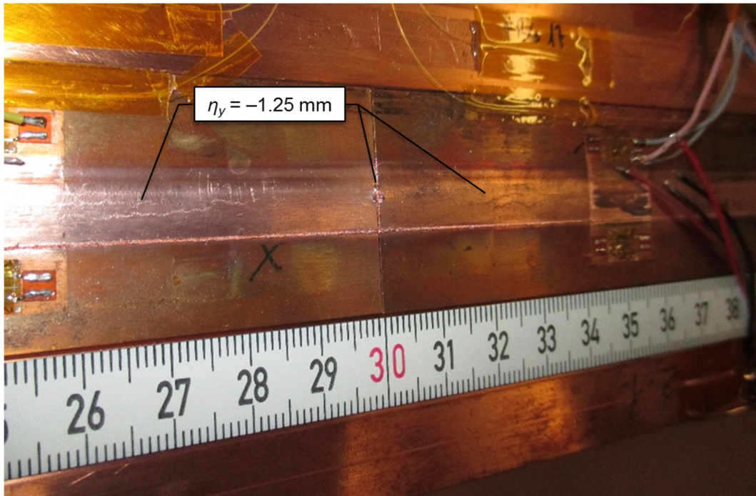
Figure 104. Impacts #45 and #46 . Note the cracks generated on the free surface of the jaw and the damage at the block/block contact.
