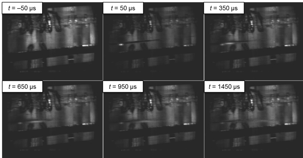
Figure 101. Micro-jetting and micro-spallation of the CuCD jaw under the impact #39 (48 bunches impacting at a distance of 0.18 mm from the free surface).
