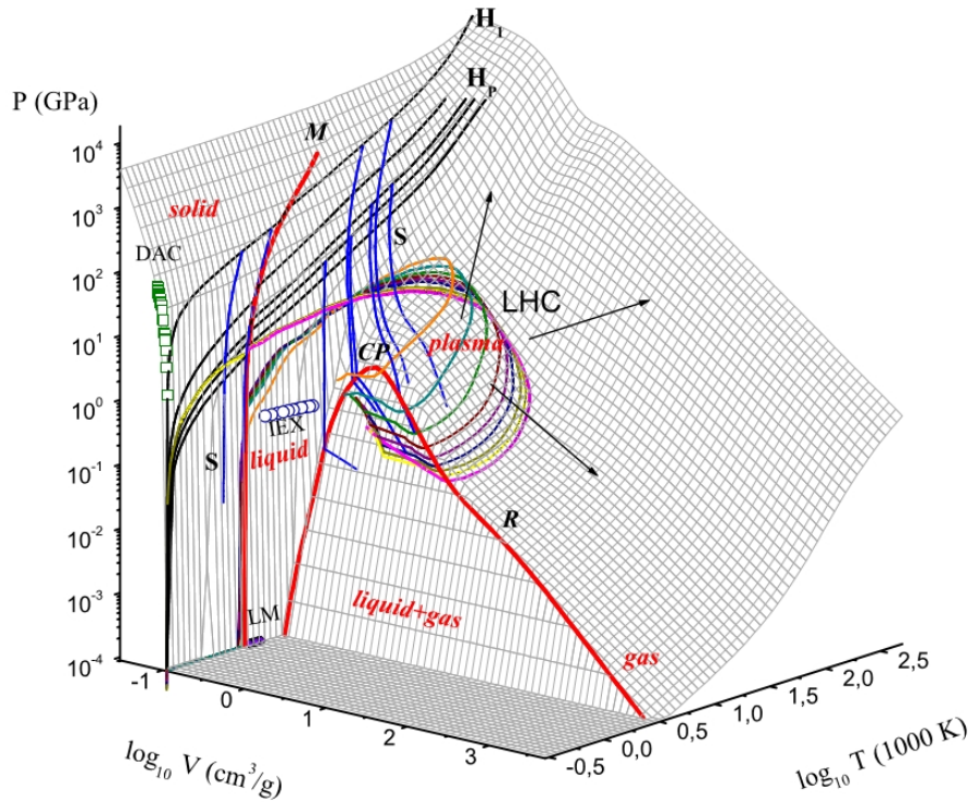
Figure 41. 3D p - v - T surface for copper. Source: [9]. M , melting region; R , evaporating region with the critical point, CP ; solid, liquid, gas, liquid+gas, and plasma (arrows indicate the decrease in plasma nonideality parameter) physical states; H1 and H_p , principal and porous Hugoniot; S , release isentropes of shock-compressed metal; IEX , isobaric expansion; DAC , static compression in diamond anvil cells; LM , density of liquid metal at room pressure; and LHC , states generated in copper by the LHC beam covering strongly coupled plasma region.
