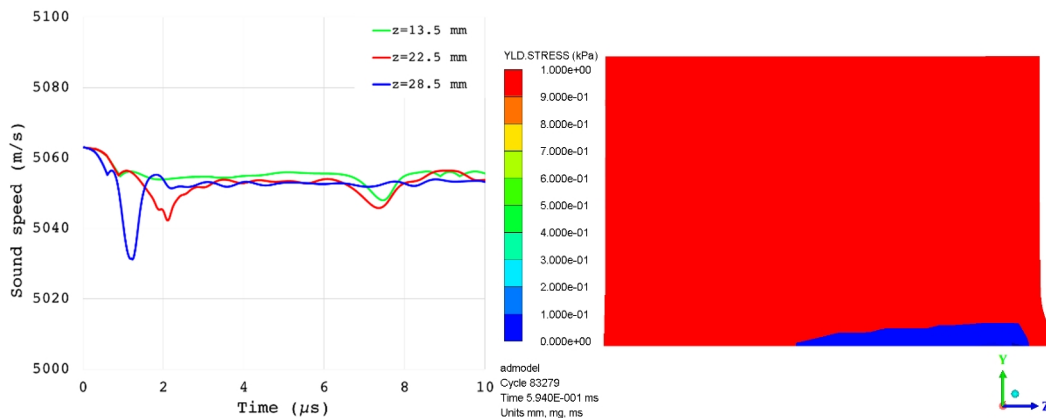
Figure 58. Left: sound speed calculated on three elements at r=0 , with different z . Right: flow stress at the end of the simulation ( t=594\mu\text{s} ) saturated at 1 kPa to show the molten material ( \sigma_y=0 ).
