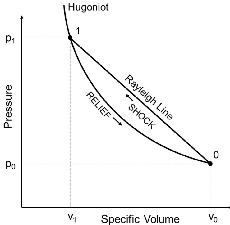
Figure 19. Characteristic Hugoniot curve and Rayleigh line in the pressure vs. specific volume plane.
