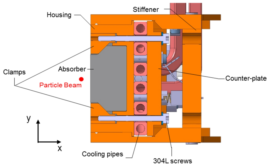
Figure 76. HL-LHC collimator jaw section.
