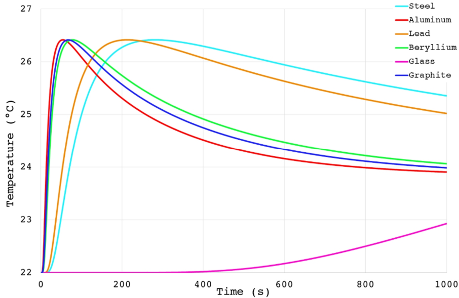
Figure 3. Temperature evolution over time on the cylindrical bar, at the longitudinal position L = 0.1 m, for different materials. The heated extremity is at L = 0 .
