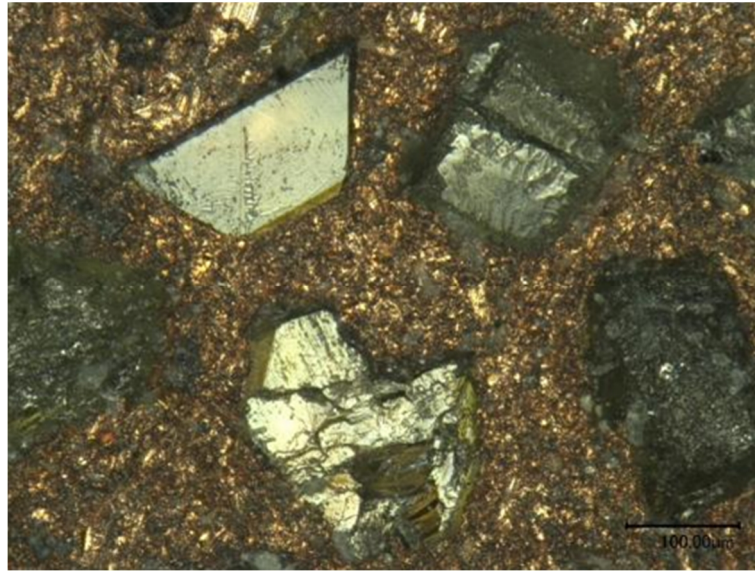
Figure 80. Optical observation of copper-diamond surface.
