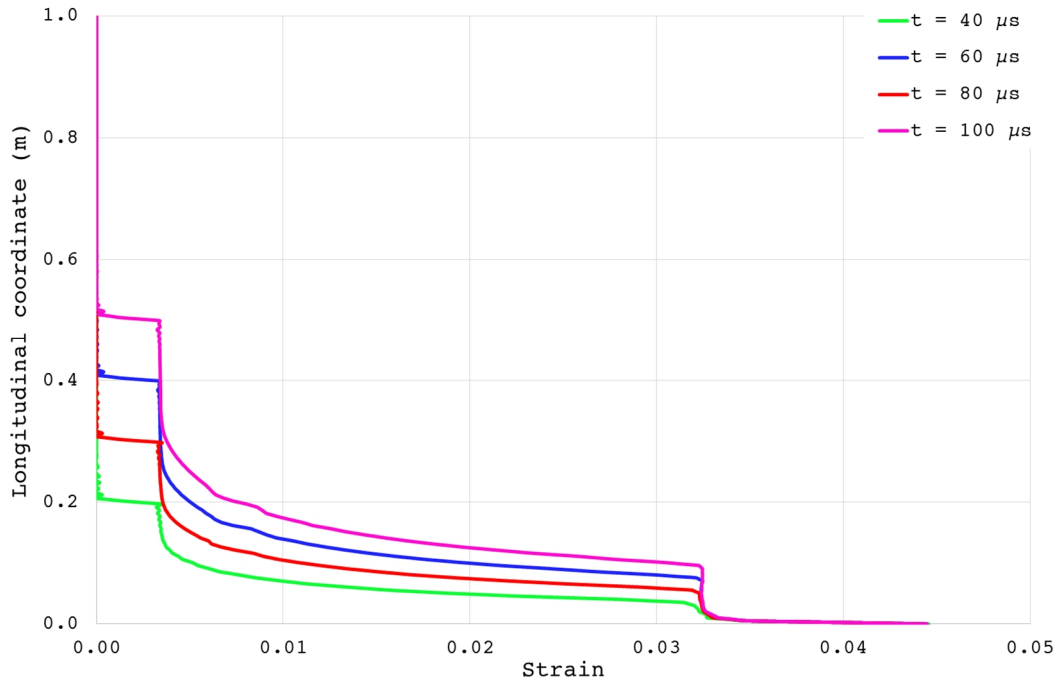
Figure 17. Plastic wave, strain profile as a function of the longitudinal coordinate x at different time instants.
