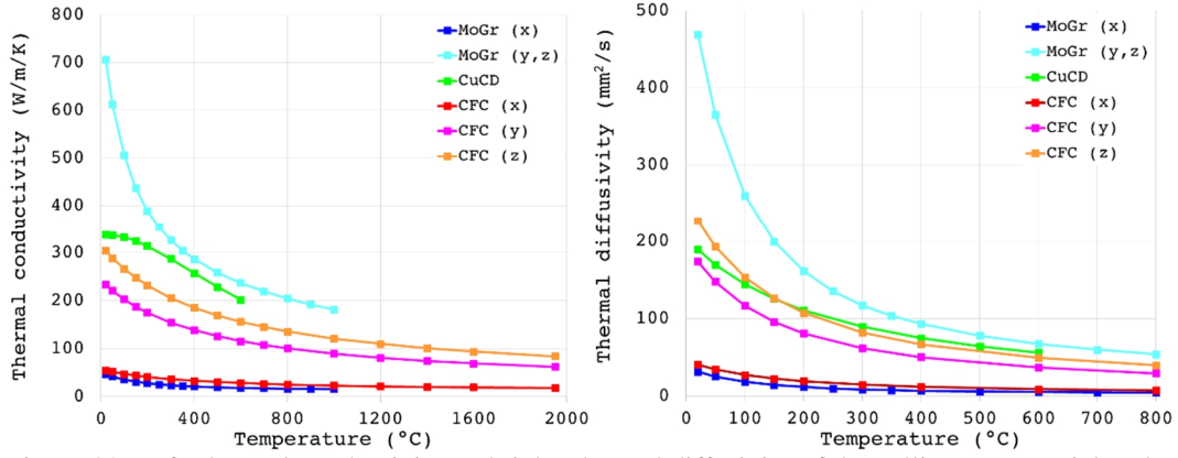
Figure 82. Left: thermal conductivity and right: thermal diffusivity of the collimator materials. The reference system is the same reported in Figure 76.
