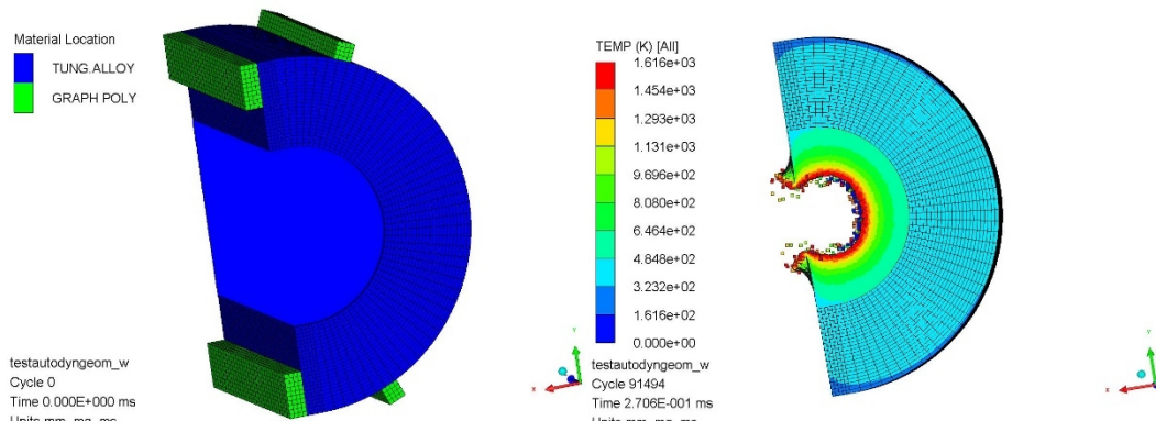
Figure 69. Left: geometry for the analysis. Diameter is 40 mm, length 30 mm; the samples have a half-moon shape, with the flat face offset by 2 mm with respect to a perfect half-cylinder. Right: H6.2 sample at the end of the simulation. The hole created by the impact is elliptical, with vertical axis 8.8mm and horizontal axis 7mm. The plastic deformation on the free surface also creates two “lips” spaced vertically by 10.1mm.
