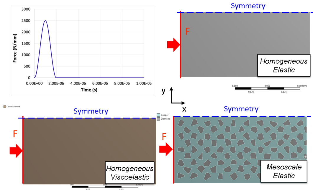
Figure 118. Homogeneous elastic (top right), homogeneous viscoelastic (bottom left) and mesoscale elastic (bottom right) models of a CuCD rod impacted at the left side with the sine excitation with half-period 2 \mu s shown on the top left. The 2D model assumes plain strain conditions.
