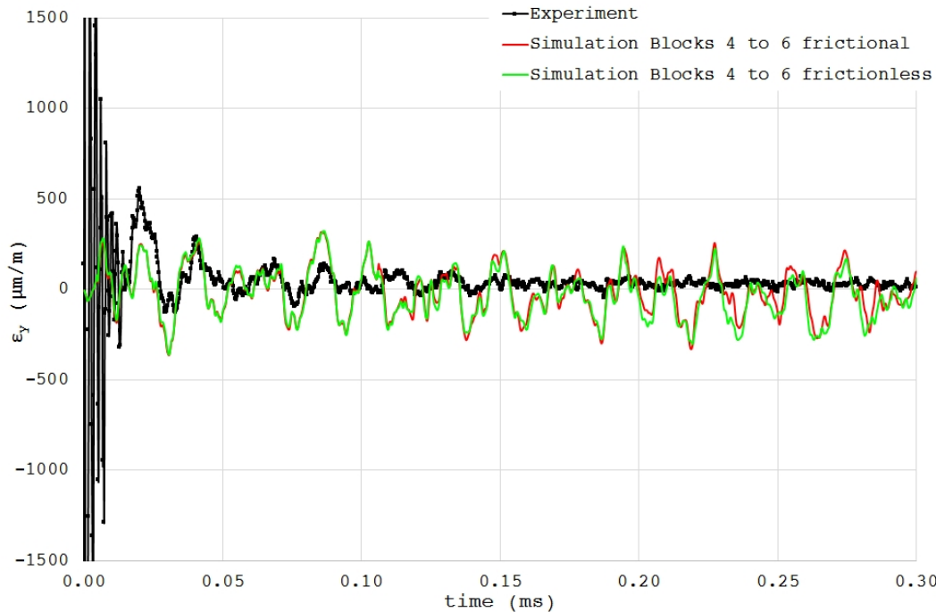
Figure 117. Impact #32 , CuCD, transverse strain on the back face of block 5: three-block model with varying coefficient of friction (frictional: c_f = 0.3 ; frictionless: c_f = 0 ).
