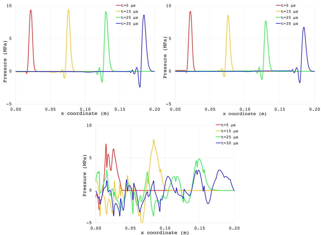
Figure 119. Pressure wave along the bar transverse coordinate in the three different models, as a response to the sine excitation with half-period 2 \mu\text{s} shown in Figure 118: homogenous elastic (top left), homogeneous viscoelastic (top right) and inhomogeneous mesoscale elastic (bottom).
