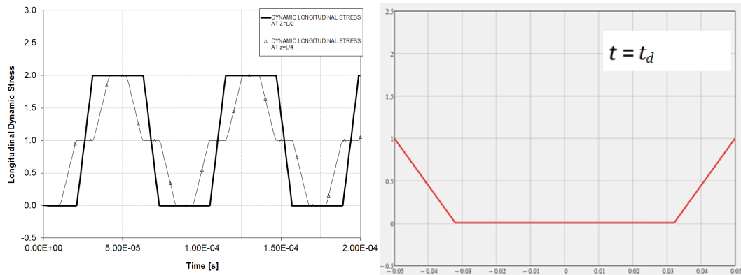
Figure 42. Left: dynamic axial stress scaled to \sigma_{ref} as a function of time at the centre and one quarter of the rod. Right: dynamic stress at the end of the deposition over the length. Source: [17].
