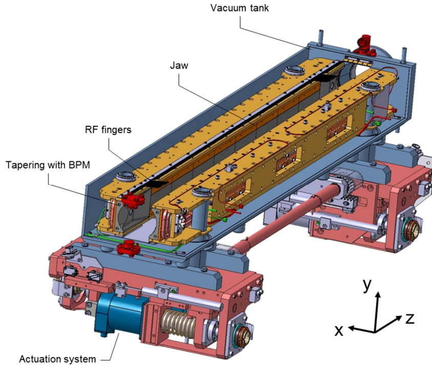
Figure 75. 3D view of the HL-LHC collimator.
