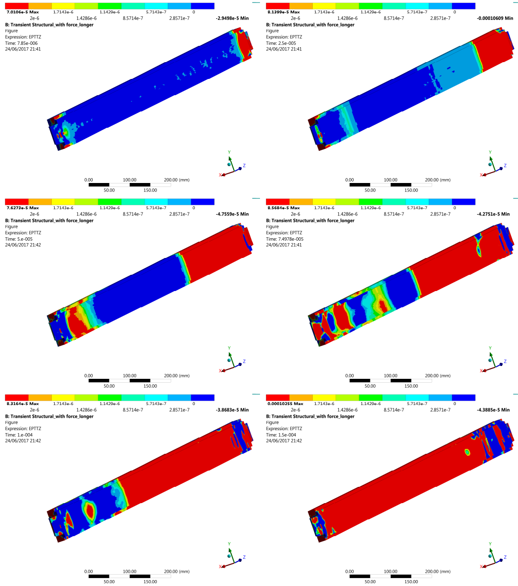
Figure 131. Impact #7, CFC : images of the total axial strain at different time instants: 7.85 \mu s (top left), 25 \mu s (top right), 50 \mu s (center left), 75 \mu s (center right), 100 \mu s (bottom left) and 150 \mu s (bottom right).
