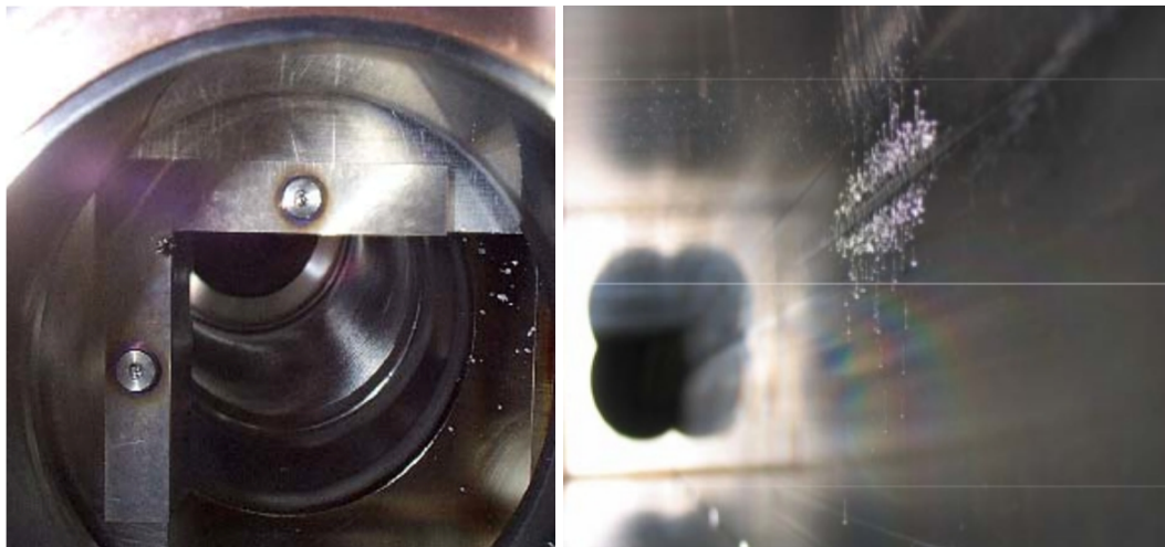
Figure 9. Tevatron collimators impacted by 1.8 MJ proton beam: tungsten (left) and stainless steel (right).
