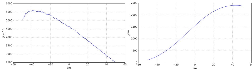
Figure 122. Left: energy peak on the MoGr absorber over the z coordinate for impact #26 . Right: total energy per longitudinal section. FLUKA maps are courtesy of E. Skordis.
