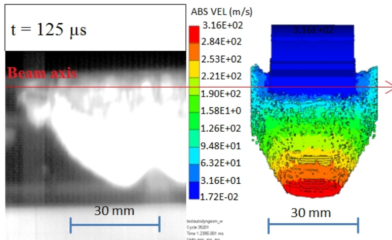
Figure 70. Comparison between acquired image and simulation of H6.2 sample 125 \mu s after the impact. On top of the specimen H6.2 , in the camera acquisition also H6.1 (first from the left) and H6.3 (first from the right) are partially visible.
