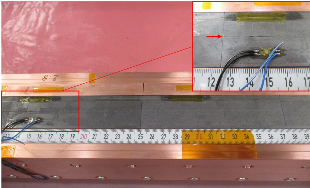
Figure 99. View of a section (between 130 and 390 mm along z ) of the MoGr jaw after extraction from the tank. Top right: zoom of the scratch at \eta_y = 0 .
