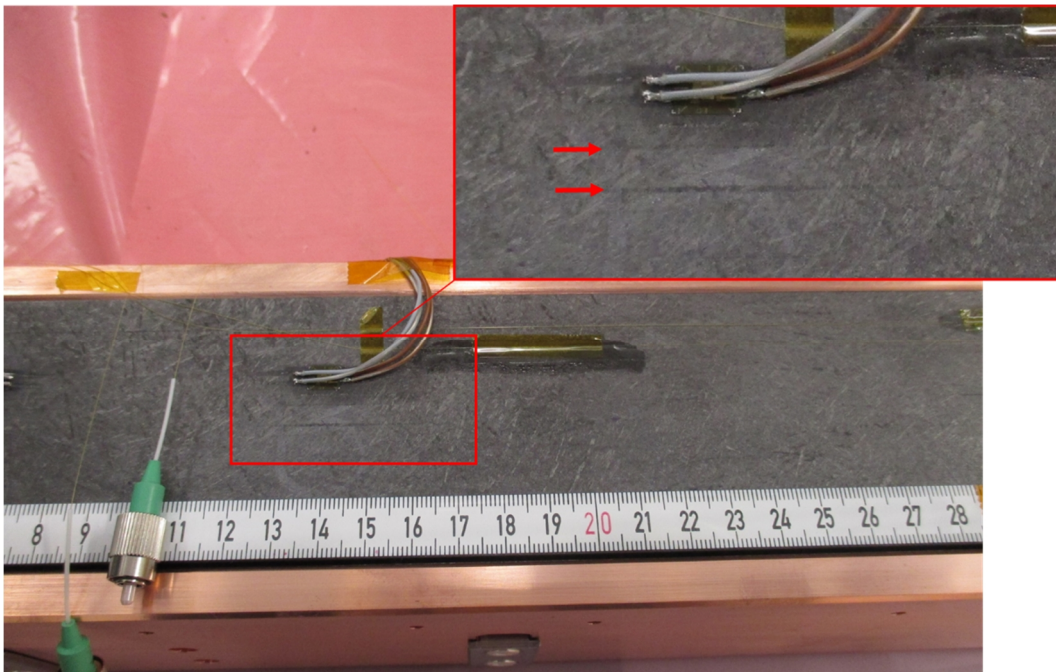
Figure 97. View of a section (between 80 and 280 mm along z ) of the CFC jaw after extraction from the tank. Top right: zoom of the two scratches at \eta_y = -2.5 \text{ mm} and \eta_y = +2.5 \text{ mm} .
