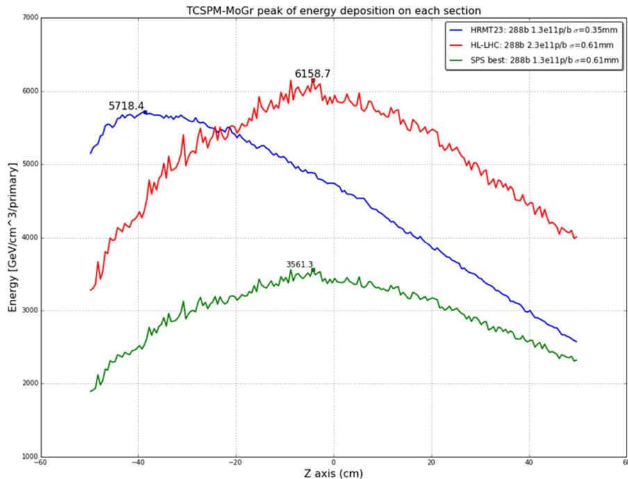
Figure 95. Comparison of peak energy depositions on MoGr for HL-LHC and HiRadMat beams. Fluka analysis courtesy of E. Skordis.
