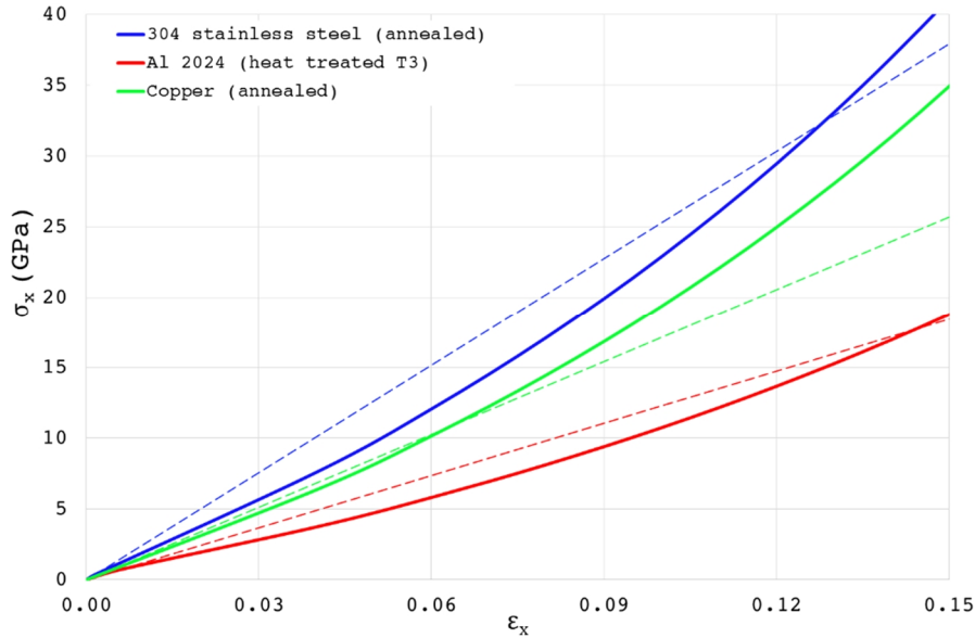
Figure 22. Hugoniot curve and Rayleigh line for three different elastic – perfectly plastic materials.
