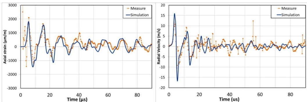
Figure 59. Left: Axial strain measurement with strain gauge at r=20\text{mm} , L=15\text{mm} vs. simulation. Right: Radial velocity measurement with LDV at r=20\text{mm} , L=15\text{mm} vs. simulation.
