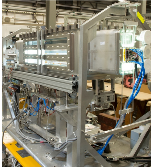
Figure 90. HRMT-23 test bench. The light for visual inspections is provided by a LED system.
