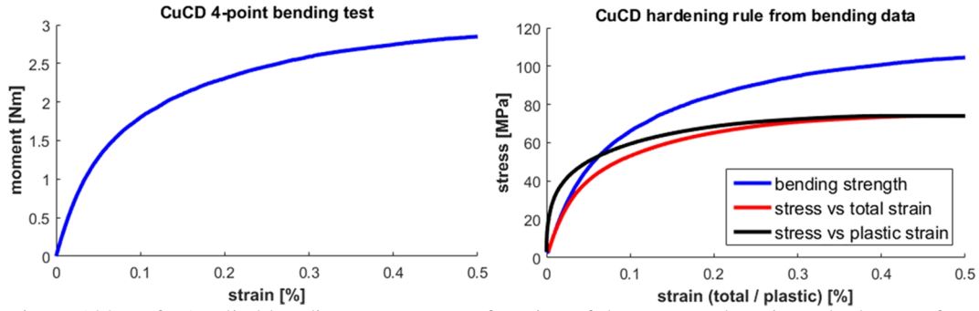
Figure 108. Left: Applied bending moment as a function of the measured strain at the bottom face of the sample. Right: flexural strength \sigma_f(\varepsilon_{max}^{tot}) (blue), the hardening curve \sigma_{eq}(\varepsilon_{eq}^{tot}) (red) and \sigma_{eq}(\varepsilon_{eq}^{pl}) (black) for the CuCD bending test.
