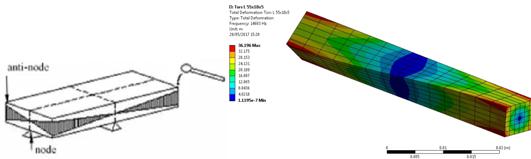
Figure 84. Left: scheme of the experimental setup for acquisition of the torsional frequencies of material plate-like specimens. Right: numerical modal analysis, first torsional mode.
