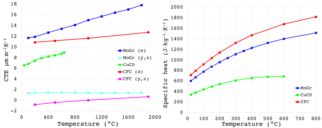
Figure 81. Left: thermal expansion coefficient and right: specific heat of the collimator materials. The reference system is the same reported in Figure 76.
