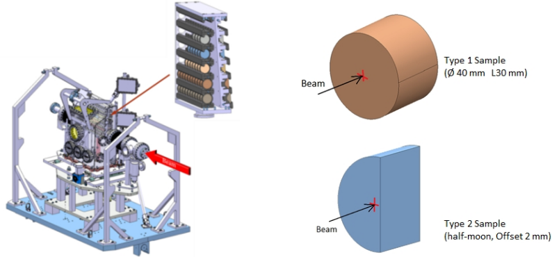
Figure 54. Left: HRMT-14 sample holder. Right: sample geometry.
