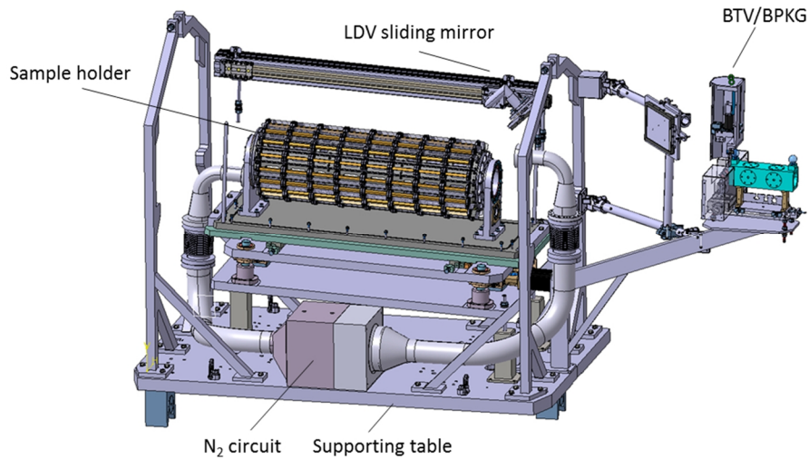
Figure 135. Inner view of the Multimatt test bench. The aluminum tank is hidden in this view. The beam comes from the right.
