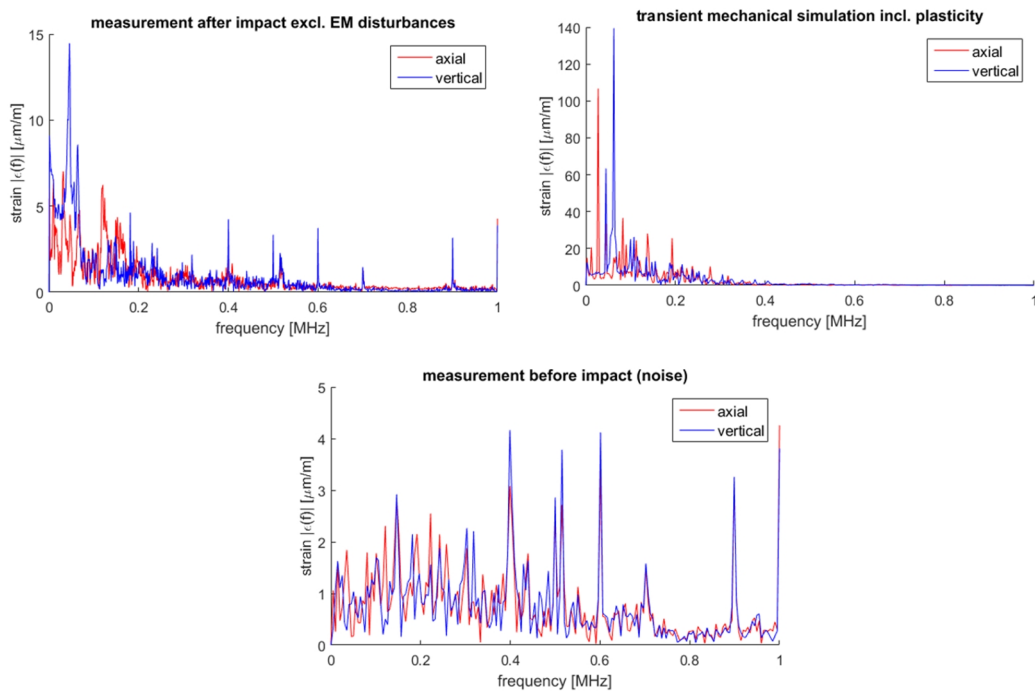
Figure 115. Impact #32 on CuCD, Fourier transform of measurement and simulation (top left and right). Note that much of the high-frequency content in the measurement signal is attributable to the intrinsic noise of the probes (bottom).
