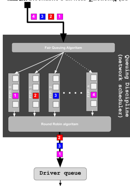
Slika 233. Stochastic Fairness Queueing (SFQ)
