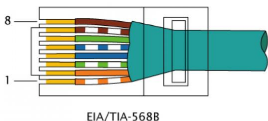
EIA/TIA-568B
