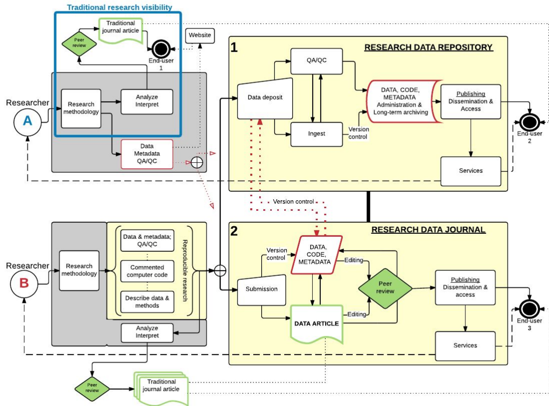
Figure 1. Research data publication workflows
