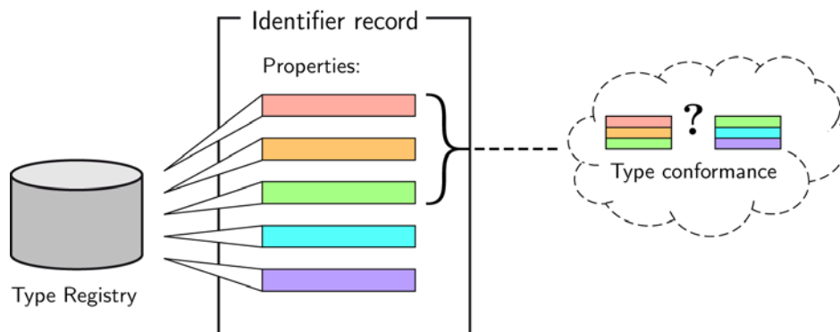
Figure 8: Relationship between a number of properties constituting an identifier record and types as aggregations of a defined set of properties. A conformance query of a specific type against a specific identifier record will then match if all of the mandatory properties of the type are present in the identifier record. Both types and properties are registered in the type registry.
