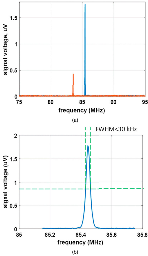
Figure 3. (A) Overlay of two NQR spectra of \text{BiPh}_3 between 75 and 95 MHz at RT (smaller, red peak) and at 77 K (larger, blue peak). The peaks correspond to the transition 7/2 \rightarrow 5/2 of Bi and appear at 83.51 and 85.45 MHz, respectively. (B): FWHM of the peak in LN, approximately 30 kHz.
