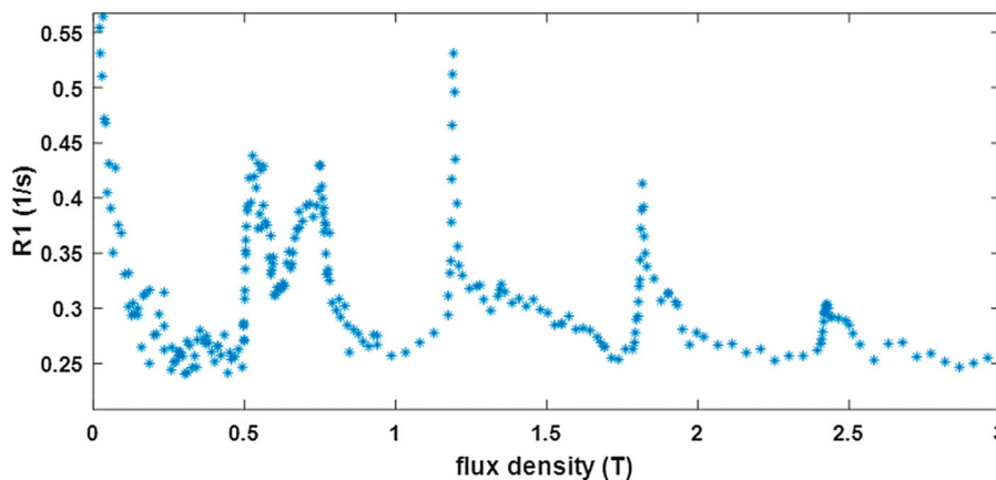
Figure 1. Example of QRE between ^{209}\text{Bi} and intrinsic protons in solid tris(2-oxymethyl-phenyl)bismuthane, see [2].
