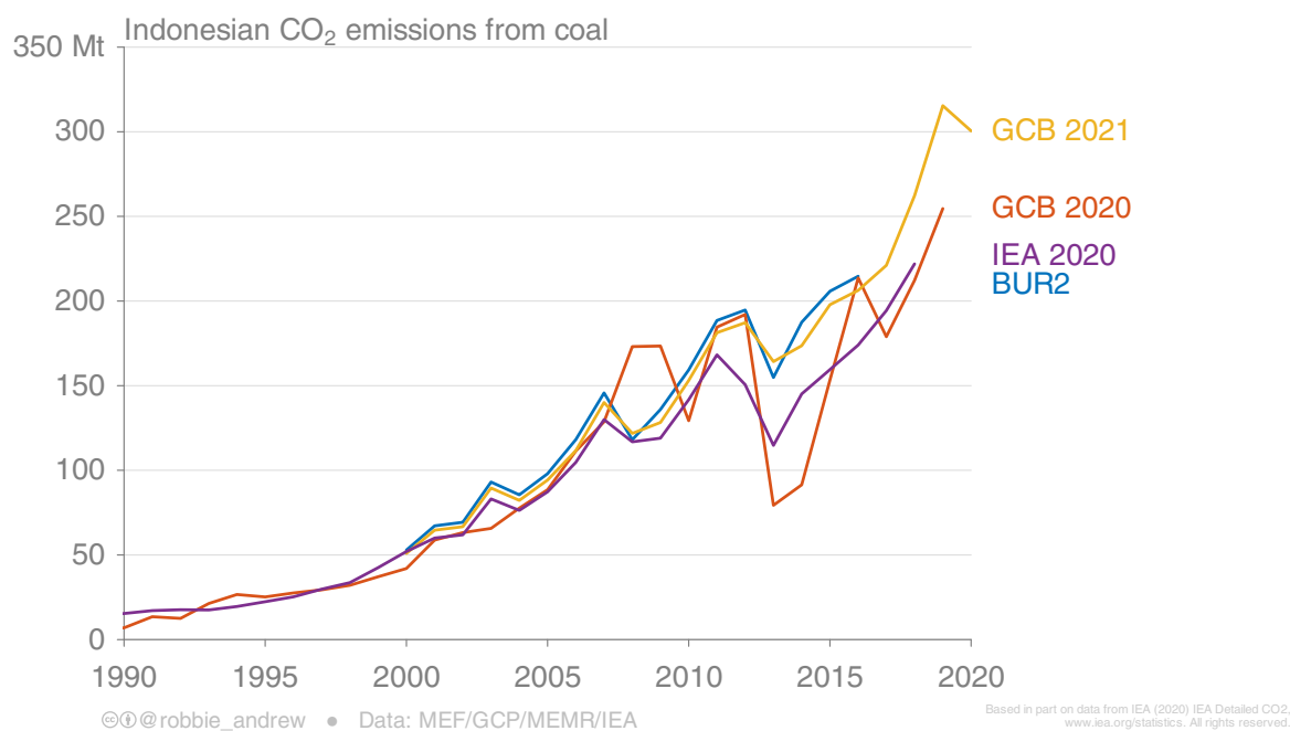
Figure 4: Comparison of Indonesia's CO 2 emissions from solid fuels reported to the UNFCCC ("BUR2"), as estimated by IEA, and as estimated in GCB before and after using data directly from Indonesia.
