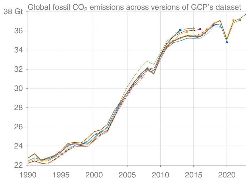
Figure 22: Comparison of global fossil CO 2 emissions from different versions of the GCB dataset. The final data point of each version is always the year before the version number, e.g., the 2024 edition has data through the year 2023 (Y-1).
