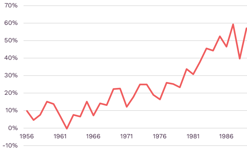
Figure 2.14 Percentage loss of total column ozone, 1956-1989 (%)
