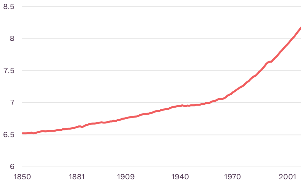
Figure 2.7 Ocean acidification by hydrogen ion concentration, 1850–2001 (nmol/kg)
