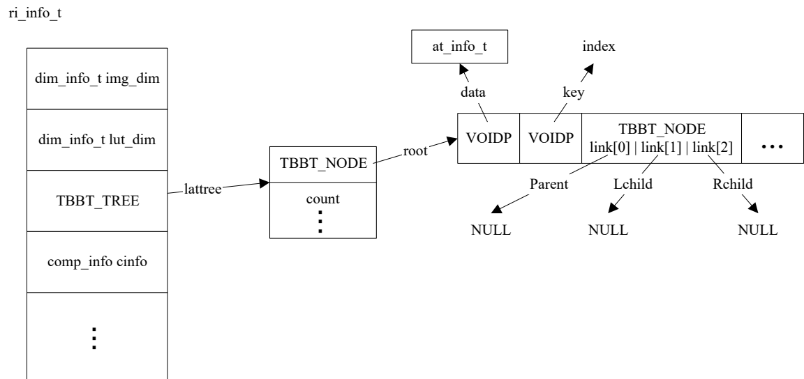
Illustration of data structure ri_info_t
