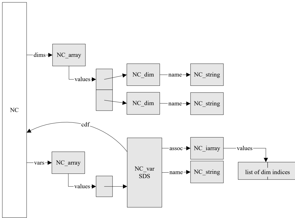
FIGURE 7r SD collection contents in memory after a 2-dimensional SDS is created
