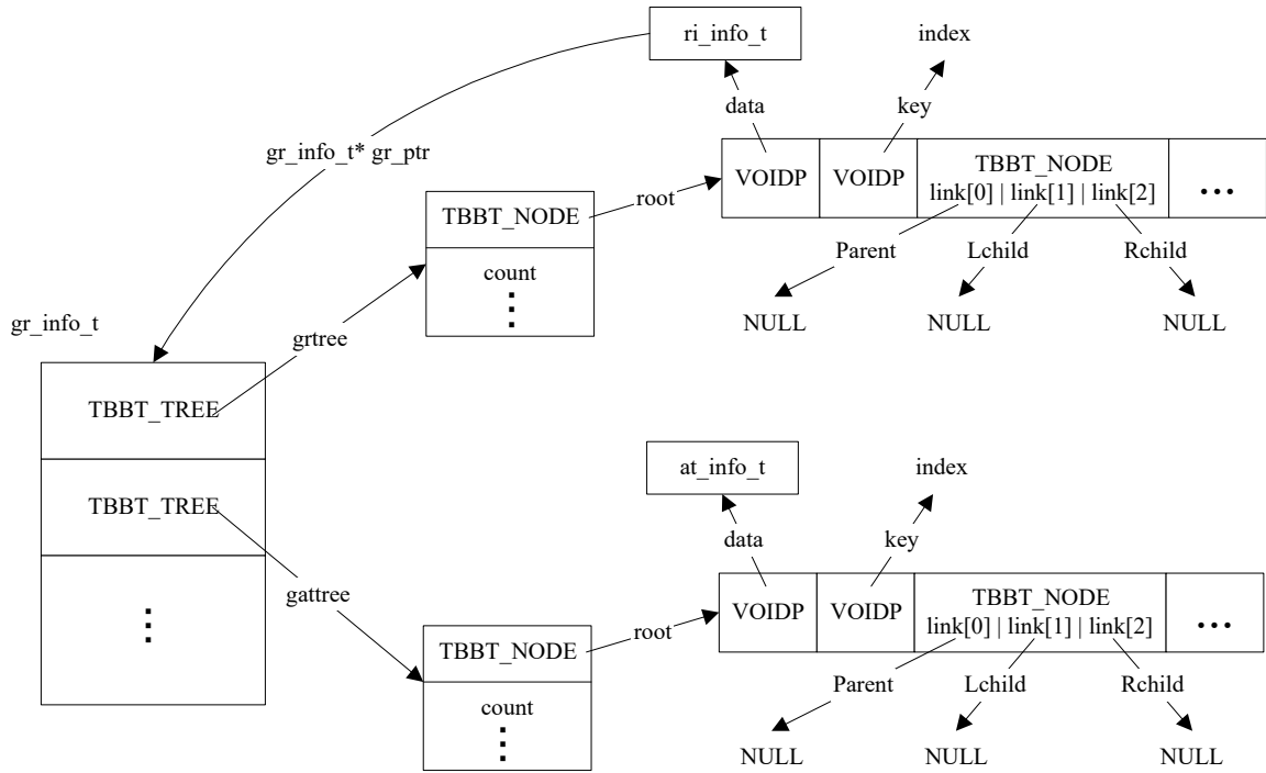
Illustration of data structure gr_info_t
