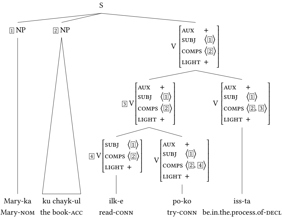
Figure 14: Clause structure with verbal complexes in Korean
