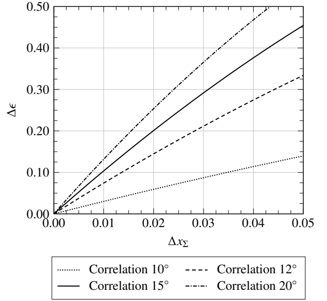
Figure 10 Estimate of Geometry-Dependent Increase in Diffuser Effectiveness (Calibrated for Numerical Data)
