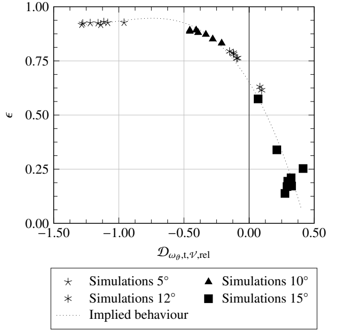
Figure 12 Correlation of Diffuser Effectiveness against Non-Dimensional Averaged Radial Diffusion of Circumferential Vorticity for Various Diffuser Half-Opening Angles from Numerical Data
