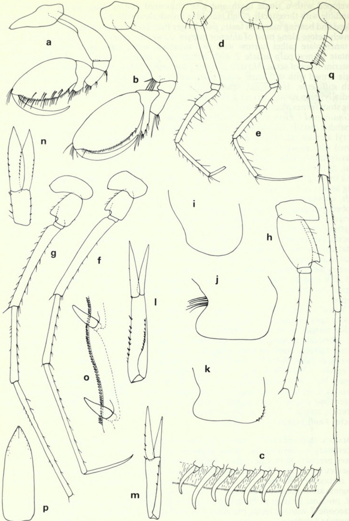
Fig. 2 Rhachotropis proxima . Male, 15mm. (a-b) gnathopods 1 & 2; (c) gnathopod 2, detail of palm; (d-h) peraeopods 3-7; (i-k) epimera 1-3; (l-n) uropods 1-3; (o) uropod 3, margin of outer ramus; (p) telson. Male, 14mm. (q) peraeopod 7.
