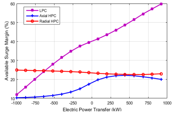
Figure 6. Available surge margin (cruise)
