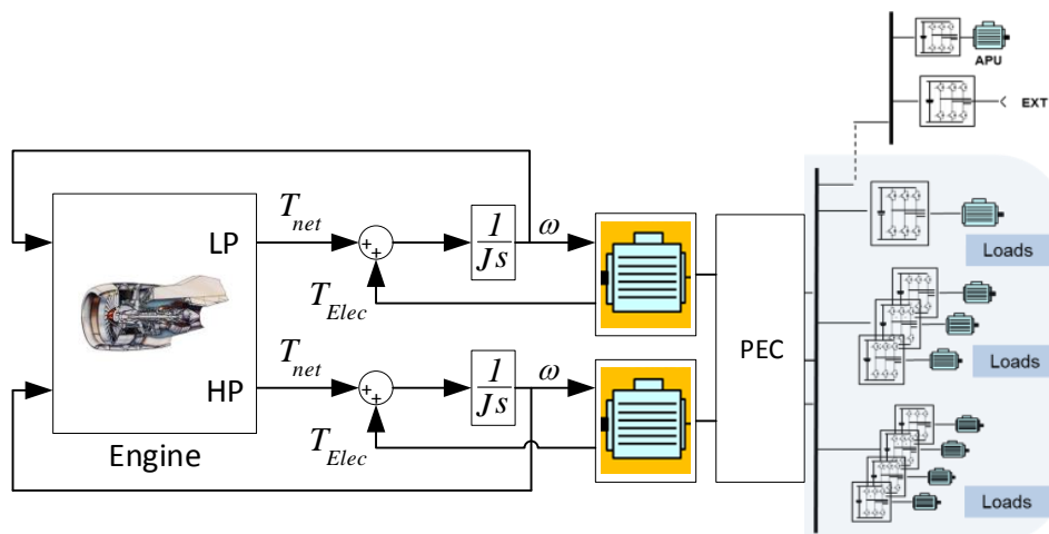
Figure 4. Schematic diagram of engine-electrical system interaction
