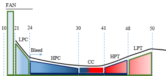
Figure 1. Illustration of turbofan components
