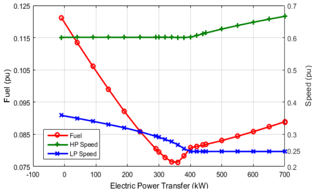
Figure 7. Fuel consumption and LP-HP speeds (ground idle)
