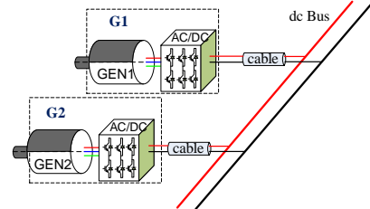
Figure 3 Configuration of single dc bus multi-source EPS
