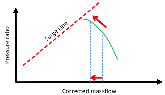
Figure 2. Operational speed line on LPC performance map
