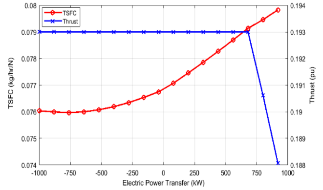
Figure 5. TSFC and per-unit thrust (cruise)
