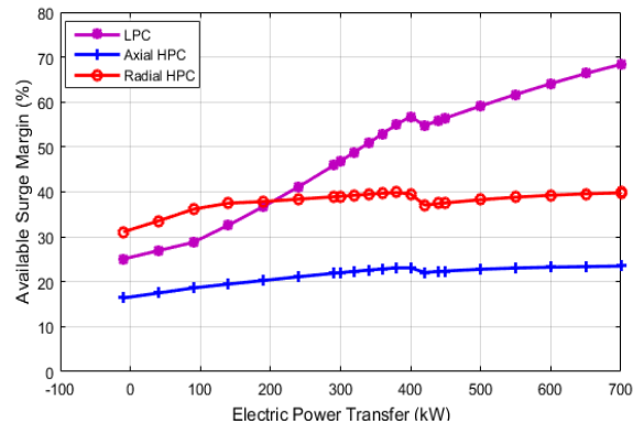
Figure 11. Available surge margin (flight idle-20000ft)
