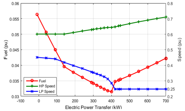
Figure 10. Fuel consumption and shaft speeds (flight idle-20000ft)
