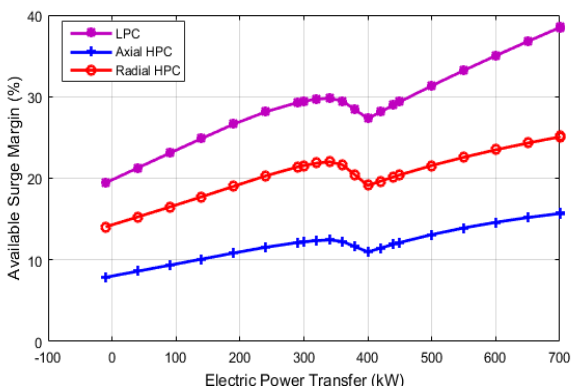
Figure 9. Available surge margin (ground idle)
