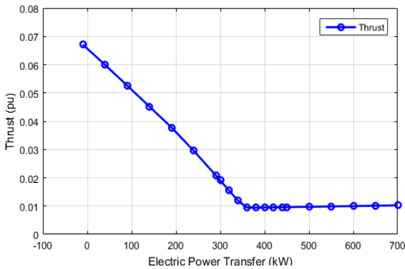
Figure 8. Calculated thrust (ground idle)
