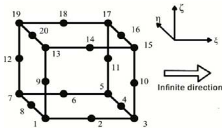
Fig. 4 20 node solid element (one infinite direction HIE)
