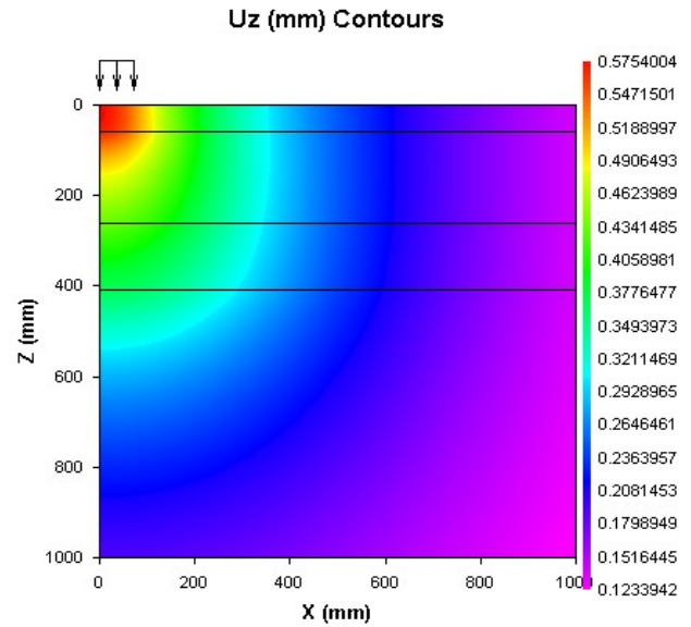
Fig. 10 Contour plot of vertical displacement
