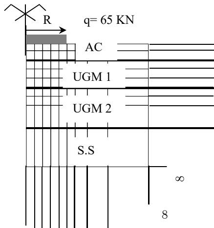
Fig. 5 Analysed pavement structure
