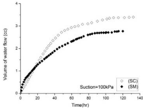
Fig. 2 Wetting curves during equalization
