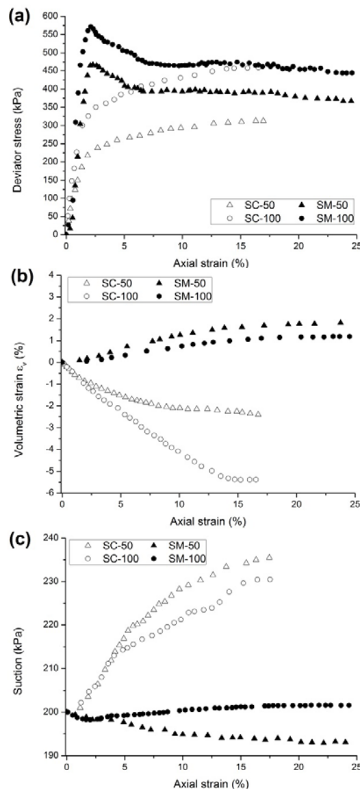
Fig. 6 (a) Deviatoric stress-strain curves, (b) volumetric strain-strain curves, and (c) suction-strain curves of CW tests at the initial matric suction of 200 kPa
