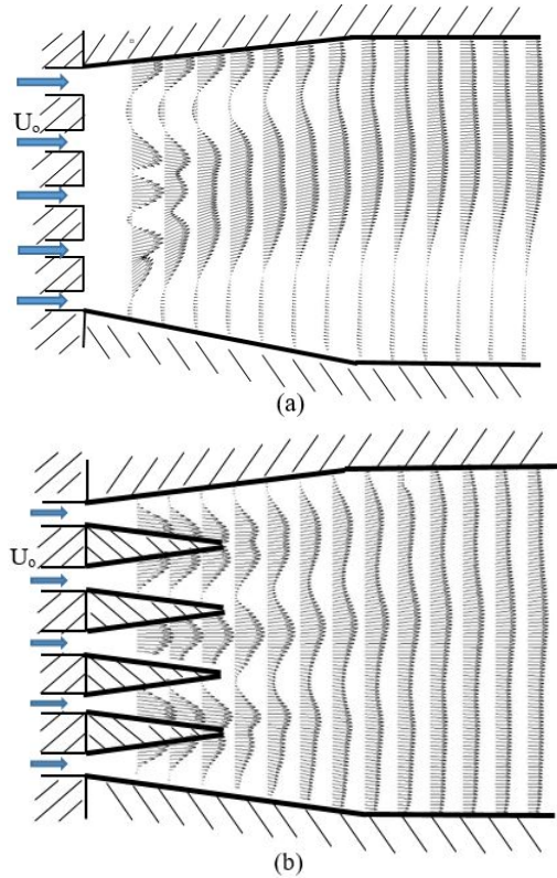
Fig. 6 Mean velocity distribution in the symmetry plane at y/w = 0.5 for the blunt geometry (a) and the triangle geometry (b) visualized with vectors
