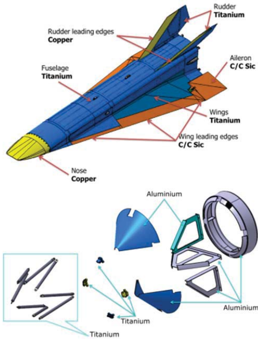
Fig. 10 Payload materials
