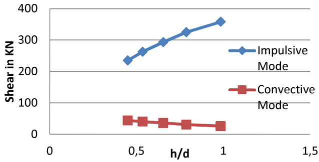
Fig. 11 Variation of Impulsive and Convective Component of Base Shear with h/d (200 KL)
