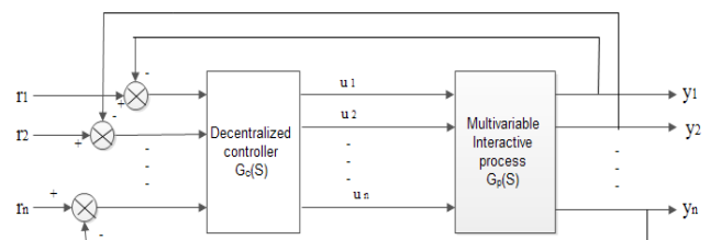
Fig. 1 Decentralized control of interactive multivariable processes
