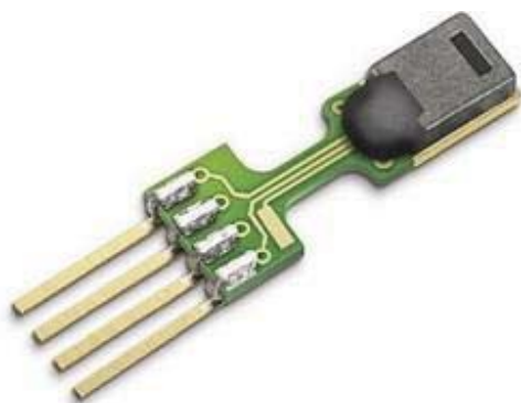
Fig. 3 (a) Capacitive sensor [13]
