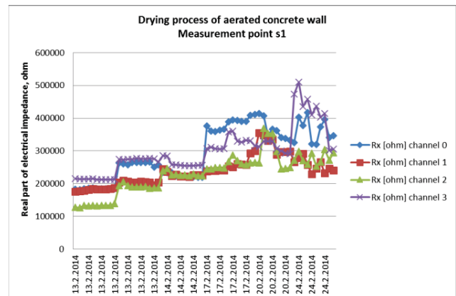
Fig. 7 Drying process of the aerated concrete wall fragment without masonry joints
