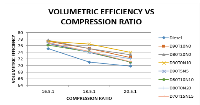
Figure 6: Volumetric Efficiency (%) Vs Compression Ratio at Maximum Torque of 24 Nm
