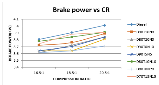
Figure 4: Brake power (kW) Vs Compression Ratio at a Maximum Torque of 24 Nm
