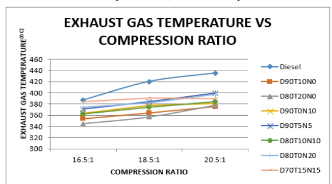
Figure 7: Exhaust Gas Temperature (°C) Vs Compression Ratio at Maximum Torque of 24 Nm
