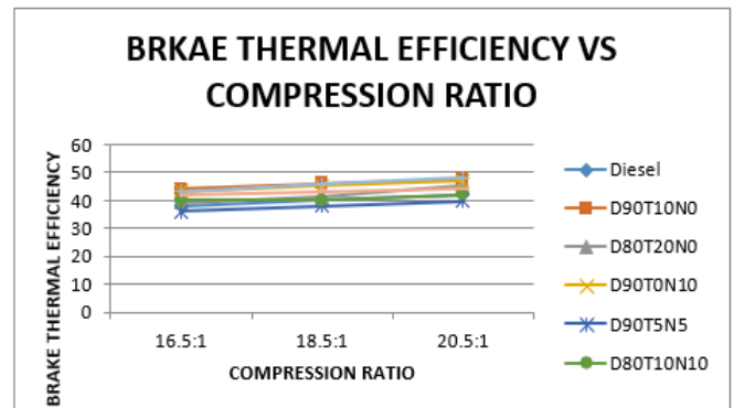
Figure 5: Brake Thermal Efficiency (%) Vs Compression Ratio at Maximum Torque of 24 Nm
